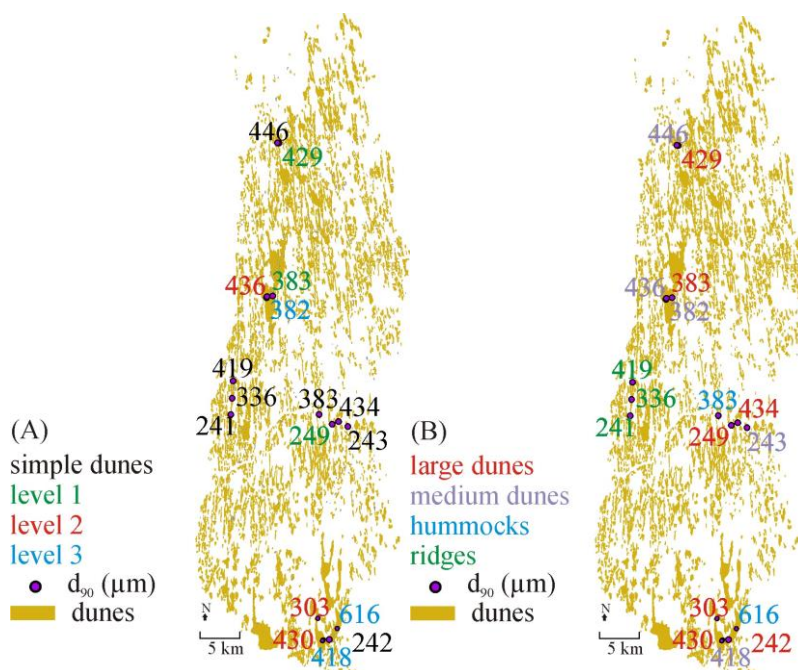
Fig. 5 The d_{90} values of the coarsest samples of the sampling sites according to the hierarchy level (A) and morphometric class (B) of the sampled dune
