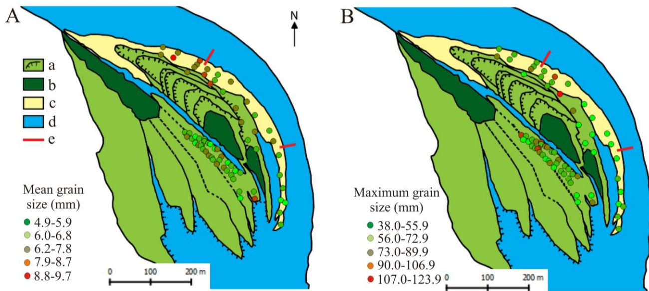
Fig. 6 Mean (A) and maximum (B) grain-size of the studied point-bar. a: slip-face of a bar; b: island-core; c: bare point-bar surface; d: water surface; e: zones of the active bar
