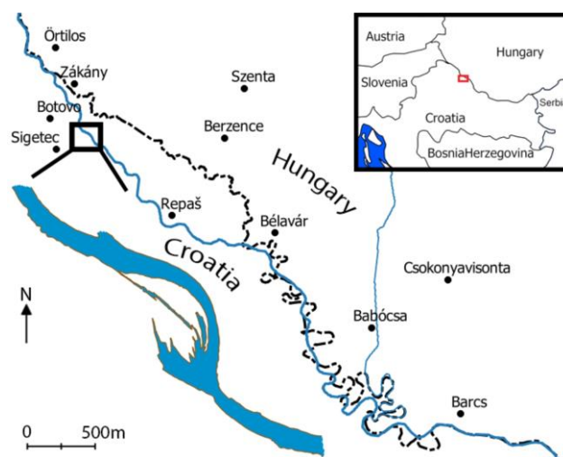
Fig. 1 The studied meander is located east of Sigetec, on the Croatian section of the Dráva River
