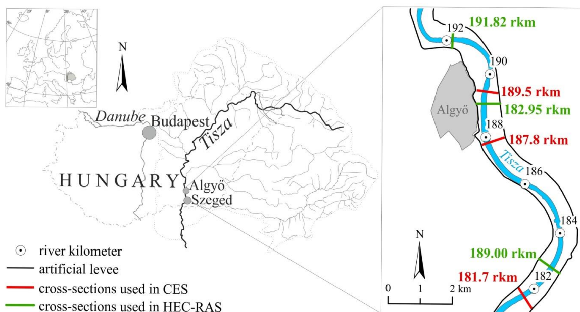
Fig. 2 Study area and the location of cross-section used in HEC-RAS and CES models
