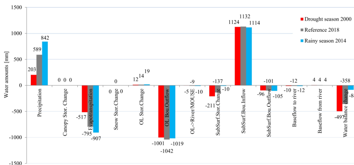
Fig. 4 Water balance values accumulated from the beginning to the end of the study years
