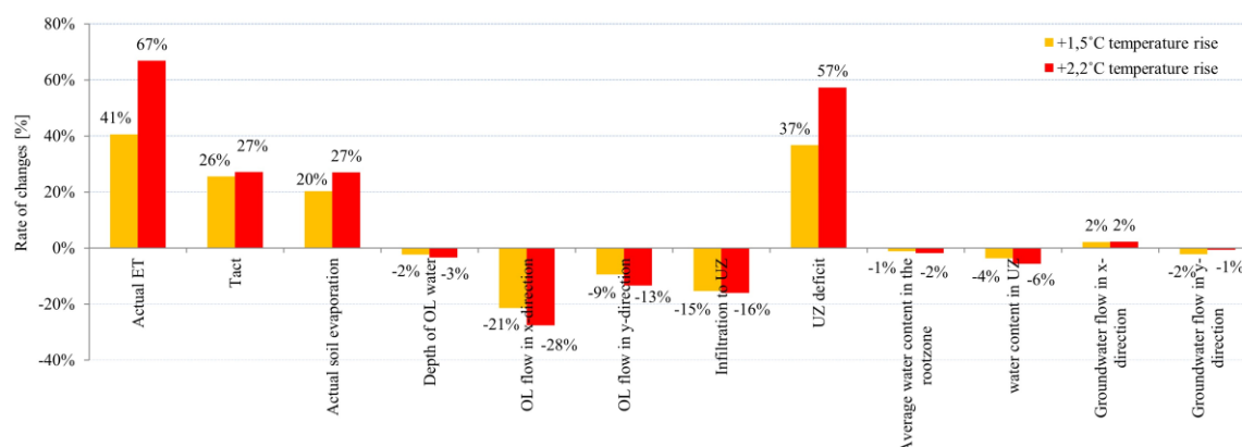
Fig. 7 Change in hydrological parameters due to temperature changes of +1.5 °C and +2.2 °C compared to the reference value on August 10, 2018 (Y = 0 horizontal axis)
