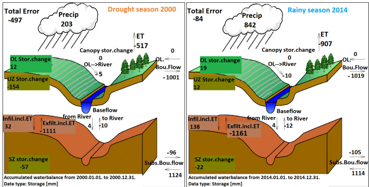
Fig. 5 Water balances for the 2000 drought and 2014 rainy years (Modified after DHI, 2017)
