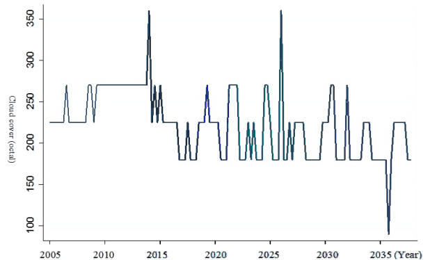
Fig. 10 Projected trend of cloud cover from 2005 to 2035
