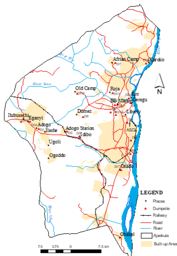
Fig. 3 Spatial pattern of existing dumpsites in Ajaokuta Sources: Sentinel-2A (February, 2021), Openstreetmap (accessed on August 25, 2021)
