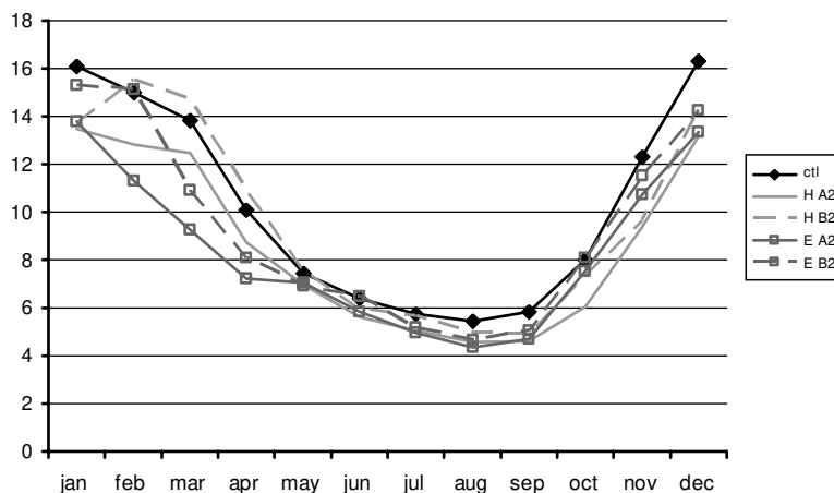
Figure 10. Median monthly streamflow in the Lake Balaton catchment ( \text{m}^3\text{s}^{-1} ): reference period (1961–1990) and future climate scenarios (2071–2100)
