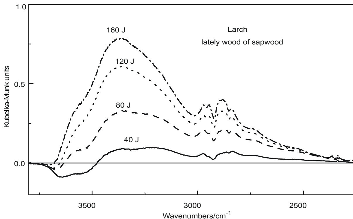
Figure 3. Difference spectra of larch (latewood of sapwood) between 3800\text{ cm}^{-1} and 2250\text{ cm}^{-1} irradiated with different impulse numbers from UV lasers
