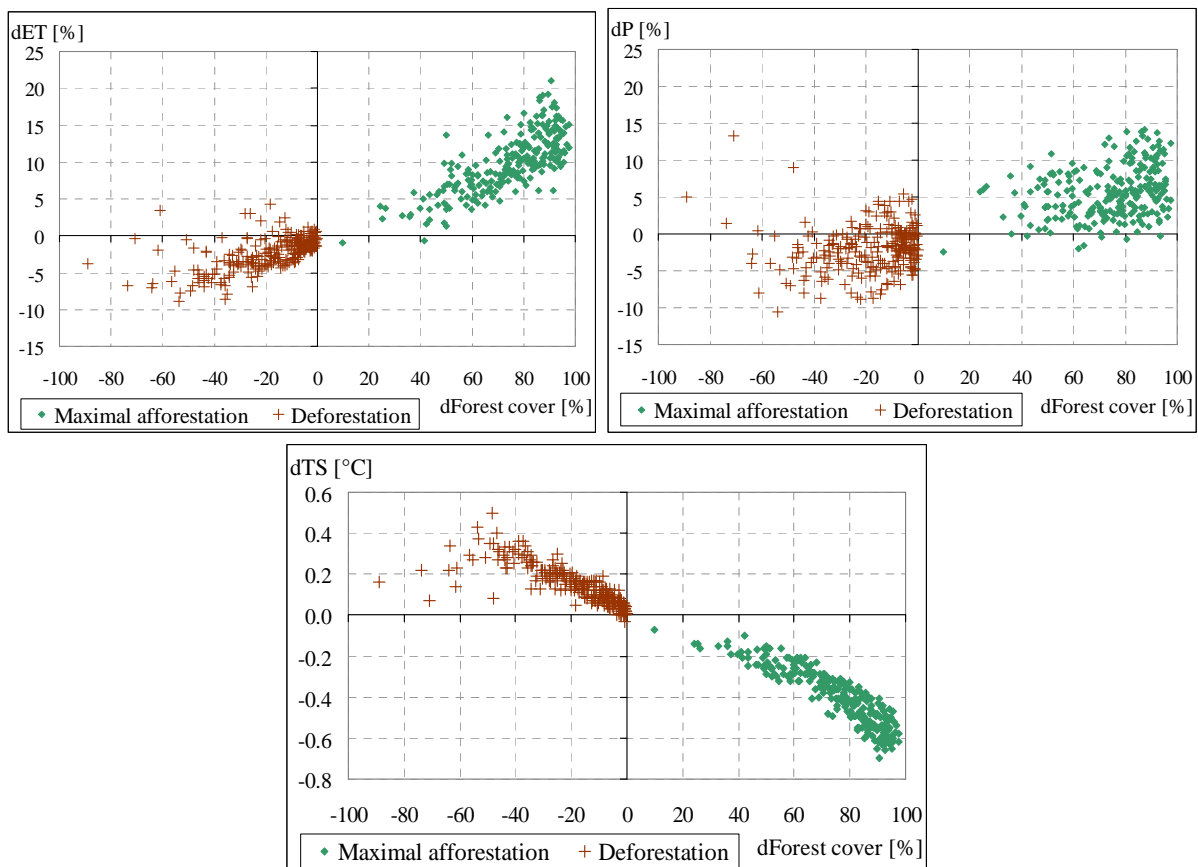
Figure 4. Correlation between the change of forest cover and the change of evapotranspiration (dET; top left), surface temperature (dTTS; bottom), and precipitation (dP; top right) for all grid boxes in Hungary in the period 2071–2100
