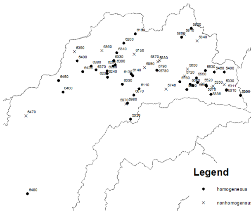
Figure 2. Map with locations and station number of homogeneous and nonhomogeneous stations at a 95% level of significance in the Vah River basin
