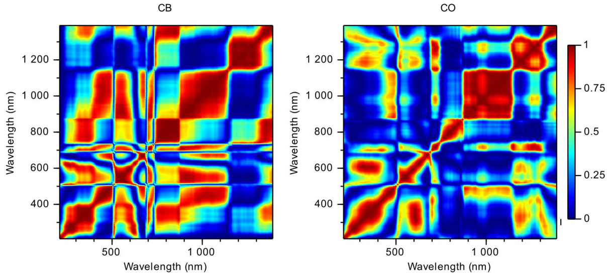
Figure 3. Two examples of autocorrelation ‘maps’ in the 200-1400 nm range, computed from 7 leaves of the first sampling. CB: Control Beech, CO: Control Oak. The colour shows the squared correlation coefficient ( R^2 ): more red means stronger linear correlation.
