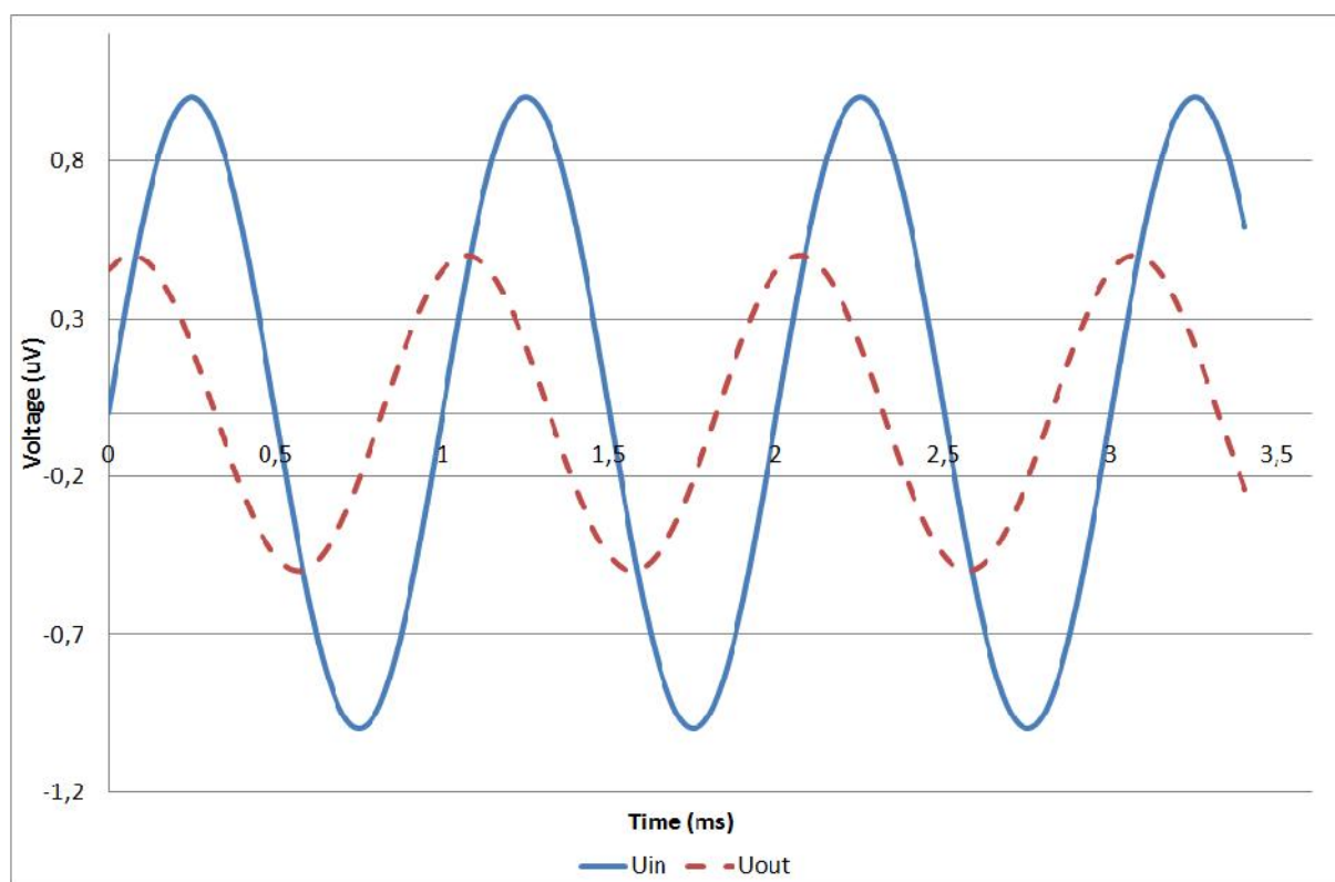
Figure 4. Illustration of the difference between the measured and reference voltages measured in linear material
