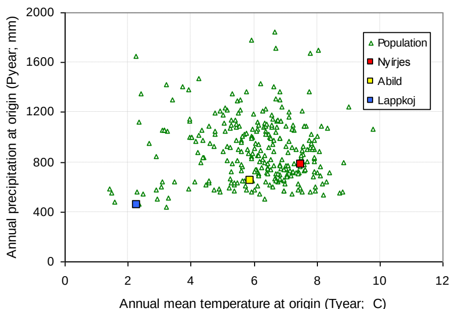
Figure 16. Climatic position of provenances from blocks Nr. 7, 8, 9 in the space of annual temperature and precipitation and the climatic location of Nyírjes and of two Swedish sites (not all provenance locations are visible due to overlay)
