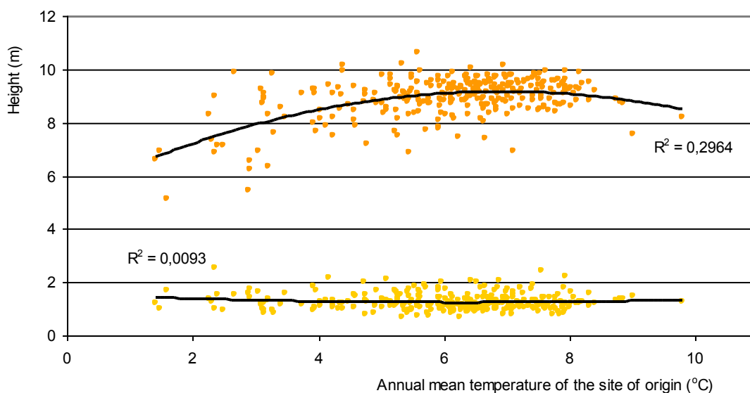
Figure 52. Average tree height (upper function) and within-population standard deviation of height (lower function) at age 16 of Norway spruce in the Nyírjes provenance test, versus annual mean temperature of the location of origin (horizontal axis)
