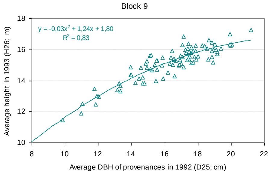
Figure 45. Polynomial regression ( R^2 ) of average DBH (age 25) and average height at age 26, determined by photointerpretation of provenances in block 9 (source: K. Czímber)
