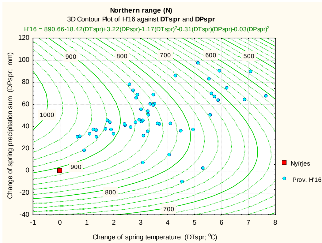
Figure 34c. Contour plot of multiple regression of adjusted height of Northern provenances at age16 ( H'16 ; cm) in Nyírjes versus ecological distances of transfer [spring precipitation change ( DP_{spr} ) and spring temperature change ( DT_{spr} )]. The reference position of Nyírjes is marked with a red quadrate. For statistical data see table in Figure 34a
