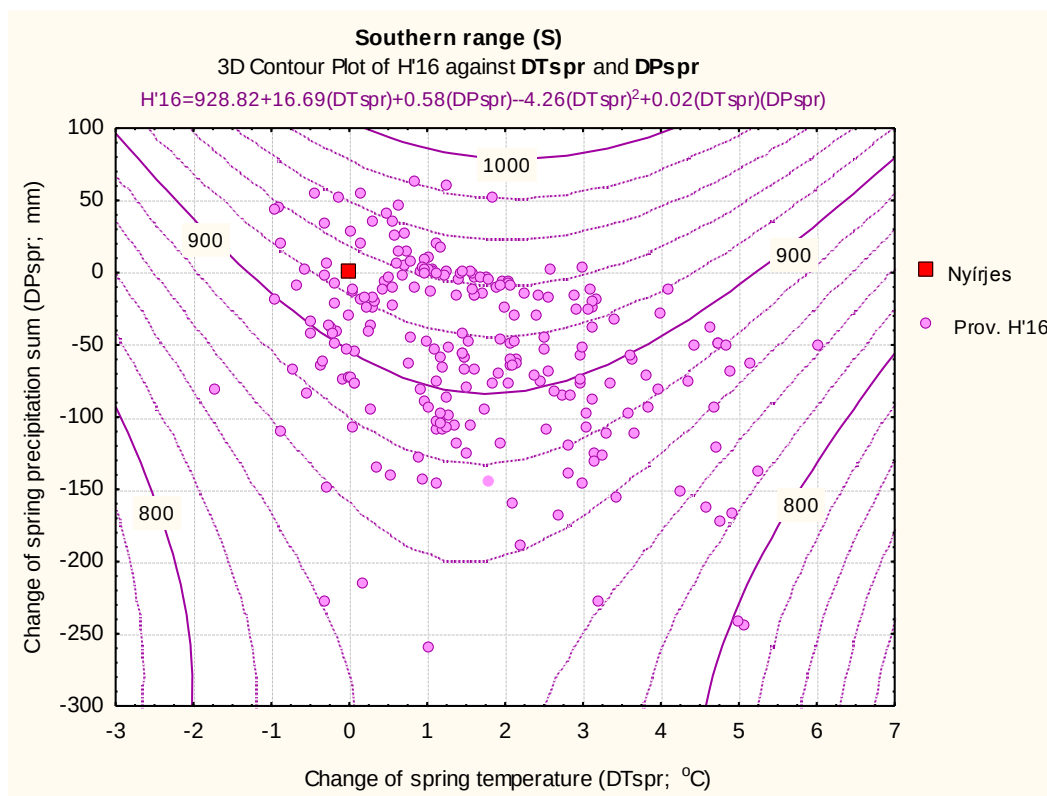
Figure 34b. Contour plot of multiple regression of adjusted height of Southern provenances at age16 ( H'16 ; cm) in Nyírjes versus ecological distances of transfer [spring precipitation change ( DP_{spr} ) and spring temperature change ( DT_{spr} )]. The reference position of Nyírjes is marked with a red quadrate. For statistical data see table in Figure 34a
