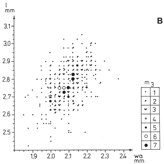
Fig. 19. Scatter diagrams of m 3 molars. A: recent material, B: Villány 8. 1-7= Fig. 2.
