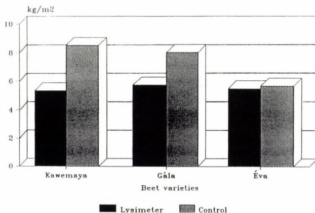
Fig. 6. Sugar production of different varieties.
