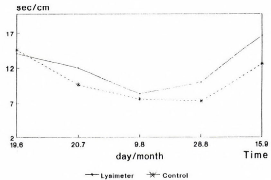
Fig. 3. Annual changes in soil surface temperature (a) and stomatal resistance (b).
