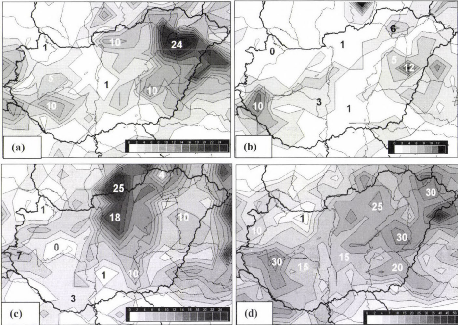
Fig. 5. Spatial distribution of severe (at least 50 dBZ) thunderstorm-ellipses in the thunderstorm season of (a) 2004, (b) 2005, (c) 2006, and (d) 2007. The resolution is 30 km × 30 km. These images were visualized by the HAWK system (Hungarian Advanced Workstation).
