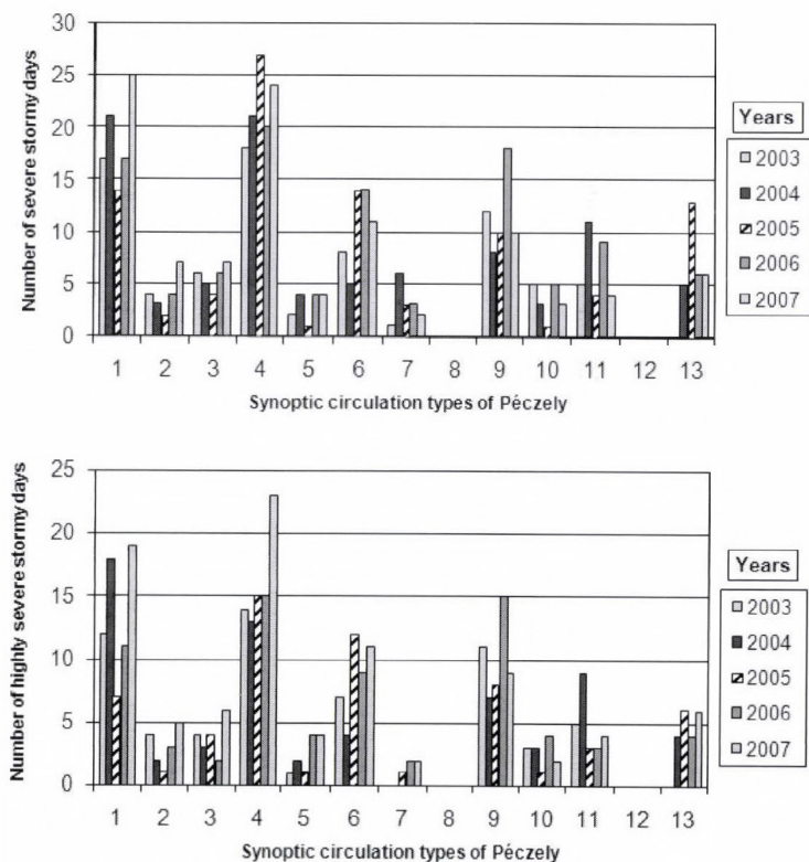
Fig. 6. Frequency distribution of (up) severe and (down) highly severe stormy days according to Péczeley's synoptic circulation types in the years 2003, 2004, 2005, 2006, and 2007.
