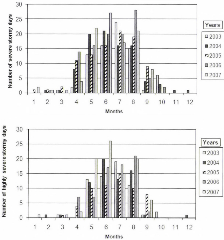
Fig. 3. Annual course of (up) severe and (down) highly severe stormy days in the years 2003, 2004 2005, 2006, and 2007. Note that in 2007 only the 9-month period from January to September was processed.
