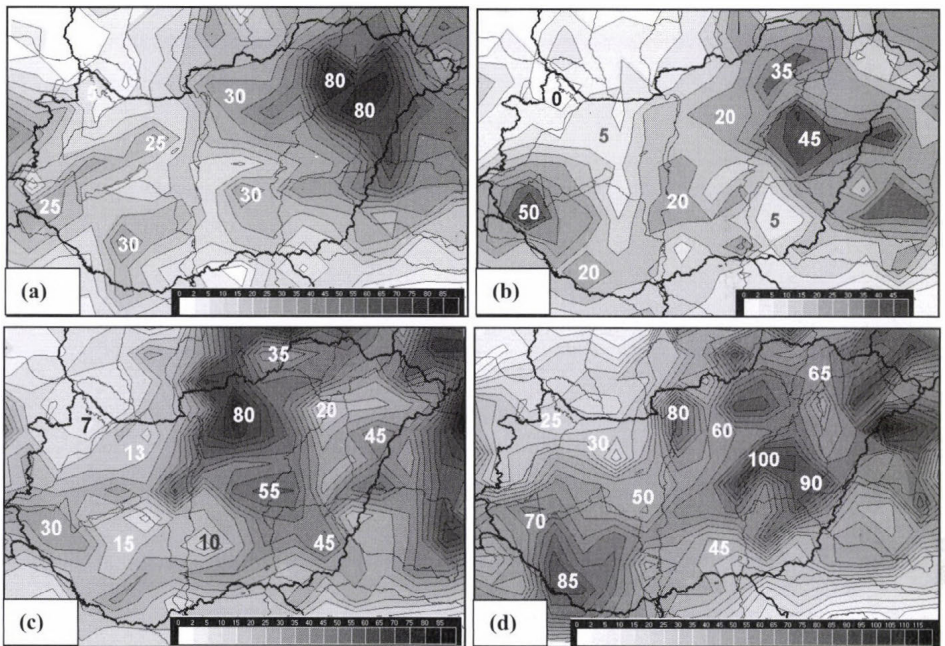
Fig. 4. Spatial distribution of severe (at least 45 dBZ) thunderstorm-ellipses in the thunderstorm season of (a) 2004, (b) 2005, (c) 2006, and (d) 2007. The resolution is 30 \text{ km} \times 30 \text{ km} . These images were visualized by the HAWK system (Hungarian Advanced Workstation).
