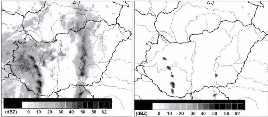
Fig. 2. Radar echo pictures of the thunderstorms observed on May 18, 2005, 14:45 UTC. Left: original picture, right: picture where thunderstorms are represented by ellipses.
