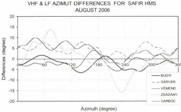
Fig. 9. Azimuth difference curves for all SAFIR HMS stations in August 2006. (The mean differences in the 0–360 azimuth were calculated between the interferometric VHF and the TOA LF positions of the same return strokes.) The azimuth error is very high for Zsadány station, it is about +/-15 degree.
