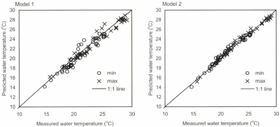
Fig. 2. Comparison of measured and predicted sets of water temperature (minimum, maximum) in 2006 (left: Model 1, right: Model 2).
