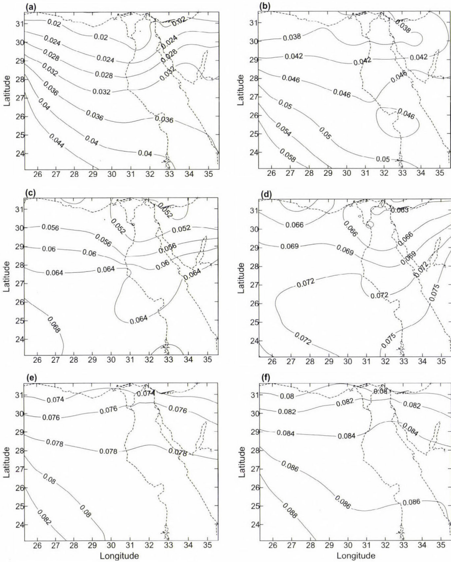
Fig. 4. The calculated UV-B values over Egypt during the months (a) January, (b) February, (c) March, (d) April, (e) May, and (f) June.
