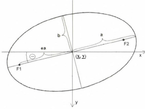
Fig. 1. Characteristics of the thunderstorm-ellipse: \bar{x} and \bar{y} are the coordinates of the centre, a is the half of the major axis, b is the half of the minor axis, F1 and F2 are the focus points, \theta is the orientation angle.
