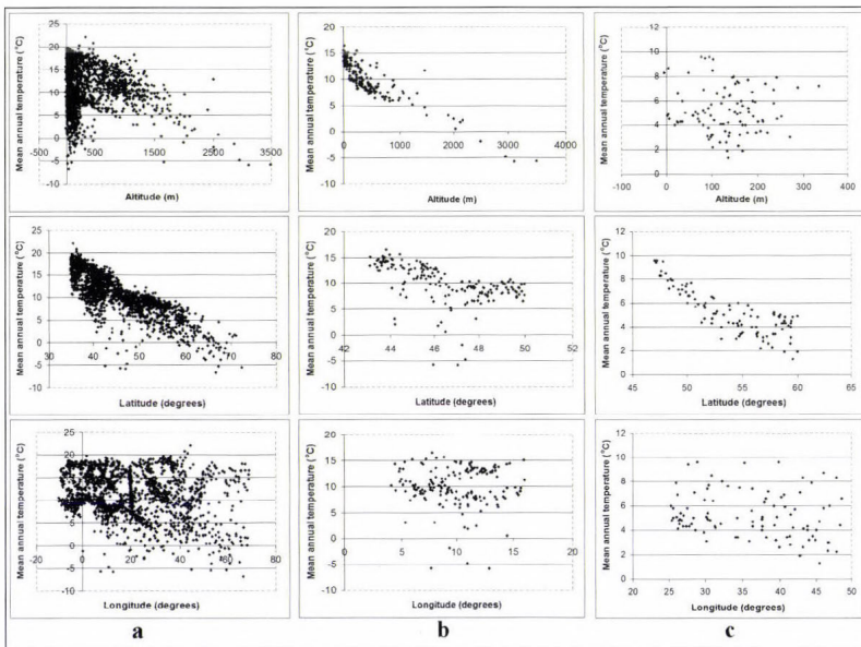
Fig. 11. Changes of the relationships between the mean annual temperatures and the altitude, latitude, and longitude for Europe (a) and for two different subregions: the Alps (b) and the Russian Plain (c). Source of data: FAO , 2003.
