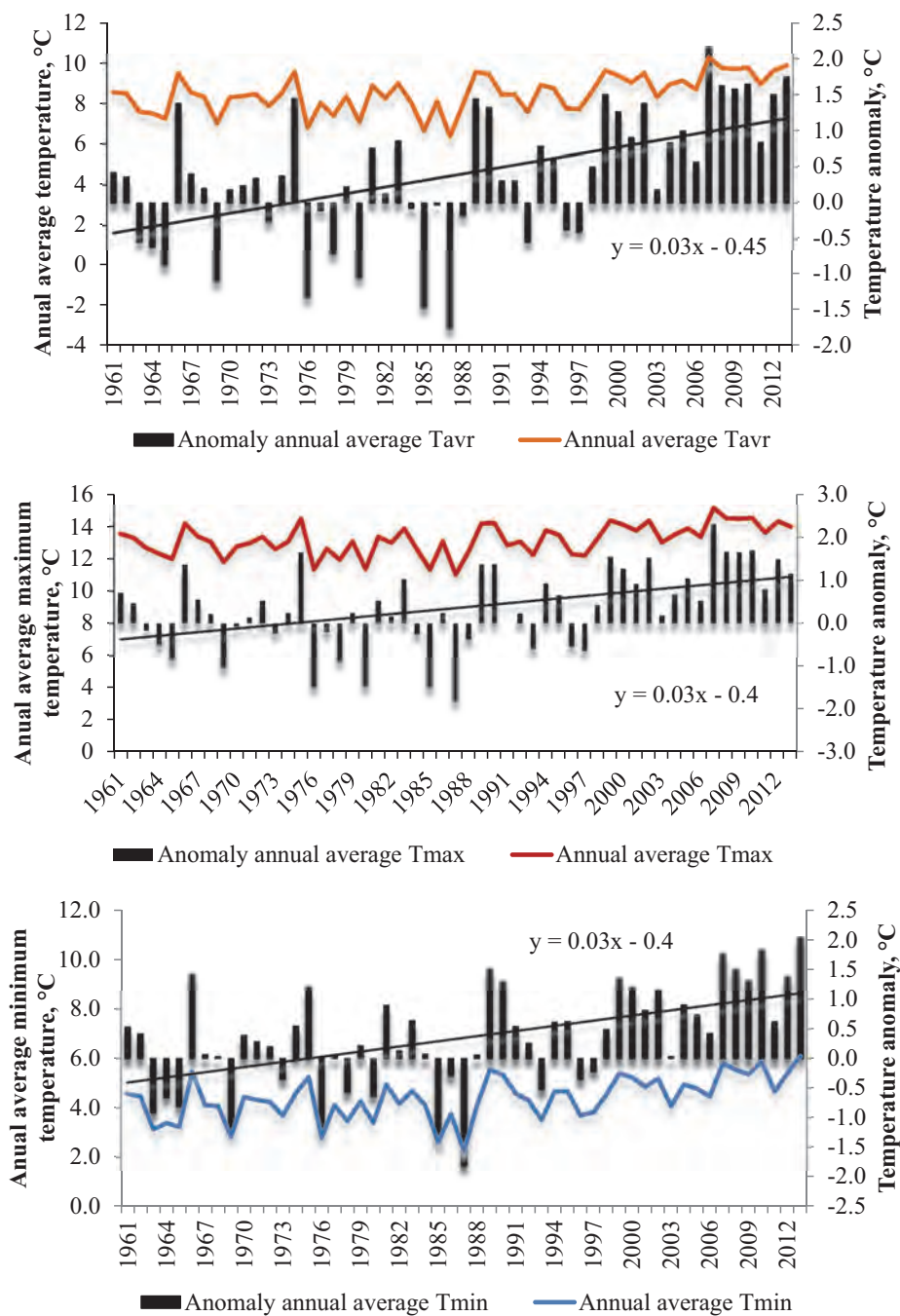
Fig. 8. Annual average (a), mean maximum (b), and mean minimum (c) land-surface air temperatures and their anomalies (°C), relatively to the climatic norm in 1961–2013, in Ukraine.
