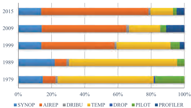
Fig. 4. The relative amounts of the main conventional data sources for the various ERA5 streams (light blue: surface, orange: aircraft, grey: buoy, yellow: radiosonde, darker blue: dropsonde, green: PILOT wind and dark blue: wind profiler observations).
