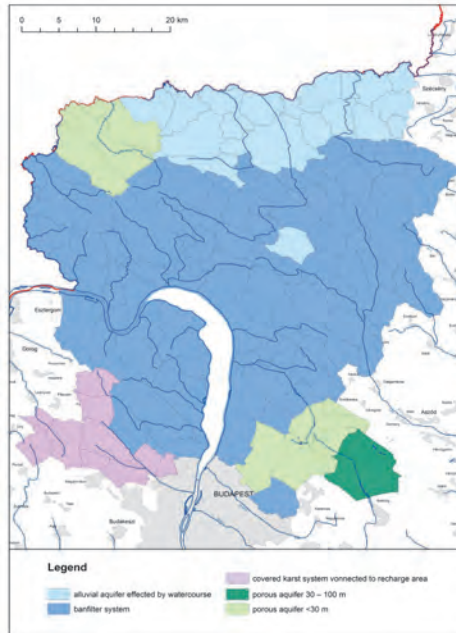
Fig. 6. Climate sensitivity of drinking water protected areas of the settlements based on the least sensitive direct water supply type, within the operational area of the DMRV.
