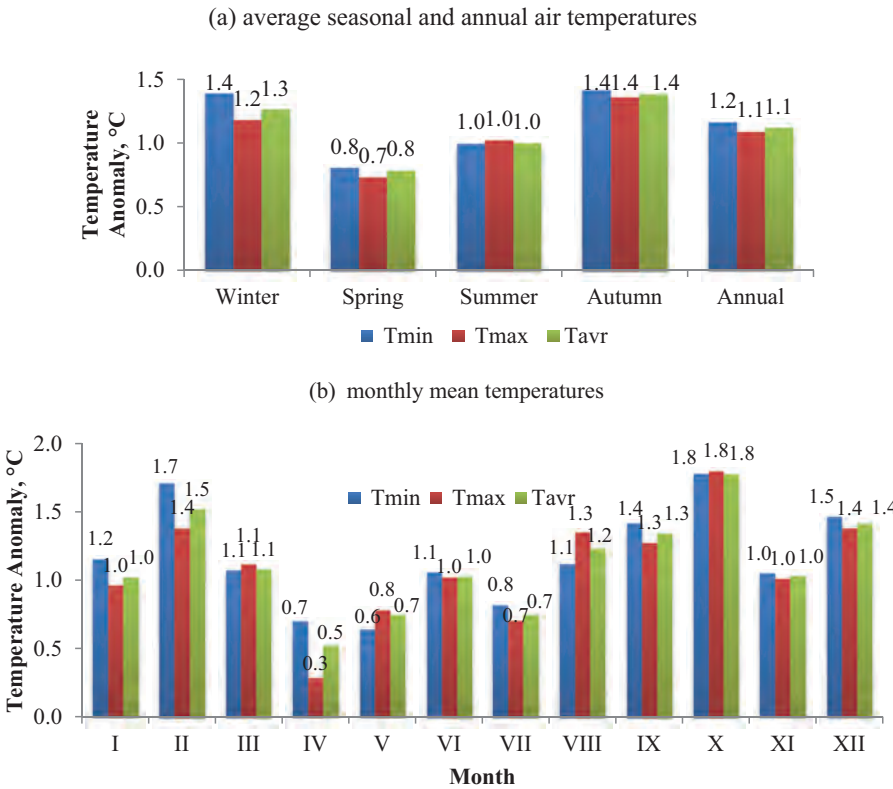
Fig.11. Projected change in the average seasonal and annual air temperatures (a) and monthly mean air temperature in 2021–2050, relatively to 1981–2010 period. Changes were calculated on the RCM REMO-ERCHAM5 model for SRES A1B scenario.
