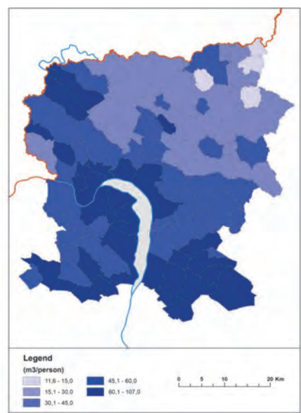
Fig. 9. The specific water consumption of settlements in the operational area of the DMRV, 2013 (Source of data: DMRV, KSH T-STAR).
