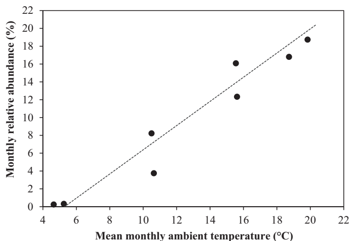
Fig. 3. The correlation between the monthly relative abundances of An. maculipennis larvae and the mean monthly ambient temperatures in March to November.
