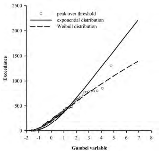
Fig. 6. Distribution of exceedances of meteo-droughts over the threshold of Z_b = 450 \text{ day}^\circ\text{C}
