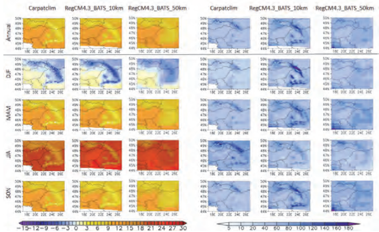
Fig. 5. Annual and seasonal mean temperature (°C) and precipitation (mm/month) of Carpatclim (left), RegCM4.3_BATS_10km (center), and RegCM4.3_BATS_50km (right), for the period 1986–2005.
