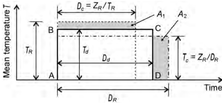
Fig. 1. Construction of the R -year design meteo-drought as proposed by Fabian and Zelenhasic (Fabian and Zelenhasic, 2016)
