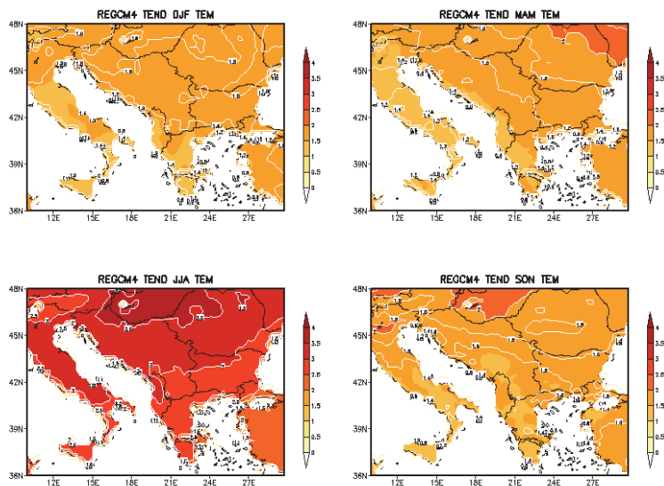
Fig. 2a. Temperature tendencies with RegCM4 model - difference between future (2021-2050) and reference (1975-2004) periods by seasons (winter - DJF; spring - MAM; summer - JJA; autumn - SON) in ^{\circ}\text{C} .
