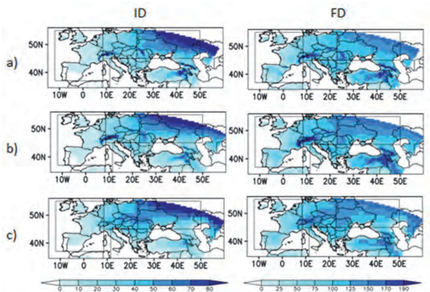
Fig. 7. Mean annual number of days of ID (left) and FD (right) in E-OBS (a, top), HadGEM2-ES (b, middle), and RegCM4.3_BATS_50km (c, bottom), for the period 1986–2005. For the sake of visual comparison, all fields are interpolated to the grid of RegCM4.3_BATS_50km.
