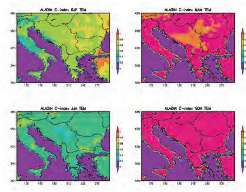
Fig. 1. Temperature C-index distribution from ALADIN model simulation for reference (1975–2004) and future (2021–2050) periods by seasons (winter - DJF; spring - MAM; summer - JJA; autumn - SON).
