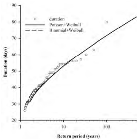
Fig. 8. Distribution of drought duration for droughts longer than 25 days
