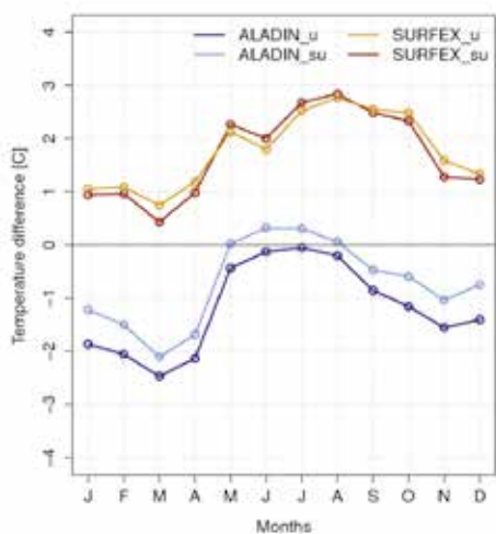
Fig. 7. Monthly 2 m temperature (left) bias of interpolated ALADIN and SURFEX and minimum and maximum temperature bias (right) of SURFEX in 2001–2010 in the urban (_u) and suburban (_su) reference points with respect to station measurements.
