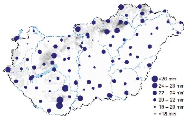
Fig. 2. 2-year return values of the 60-minute rainfall.
