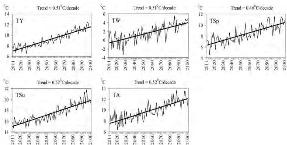
Fig. 2. Trend of the mean temperatures: annual (TY), winter (TW), spring (TSp), summer (TSu) and autumn (TA), at the significance level of p < 0.0001 , in Kolašin in the period 2011–2100 based on the A2 scenario of the EBU-POM model.
