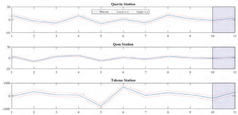
Fig. 3. Verification of simulated values by using vector autoregressive model at Qazvin, Qom, and Tehran stations.
