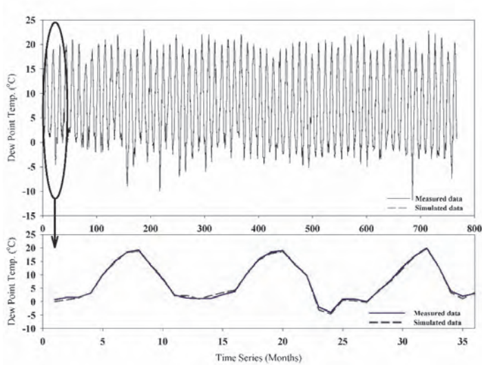
Fig. 4. Estimation of DPT values of Gorgan meteorological station using Pattern I.
