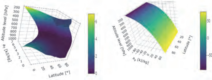
Fig. 5. The available enthalpy temperature- (left) and pressure-dependent (right) terms for the Northern Hemisphere, made by 41 years average.
