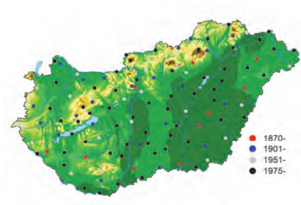
Fig. 1. Location of the stations in case of temperature.
