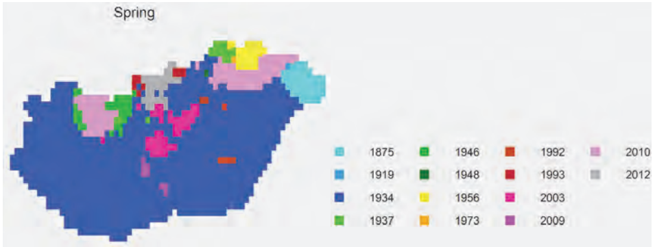
Fig. 9. Spring: year of maximum SPTI values.
