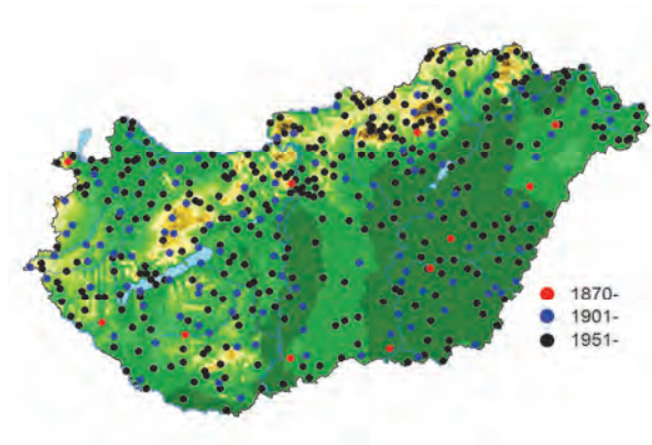
Fig. 2. Location of the stations in the case of precipitation.
