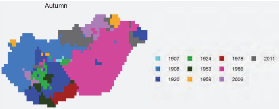
Fig. 11. Autumn: year of maximum SPTI values.
