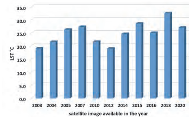
Fig. 5. Landsat mean LST evolution in the general built-up (urban) land cover over available Landsat images.
