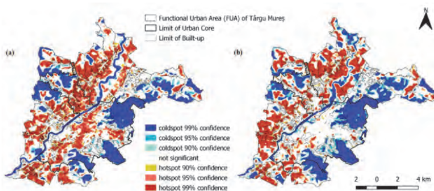
Fig. 10. Significant LST hotspots and coldspots (a) between 2003–2018 and (b) in 2020.
