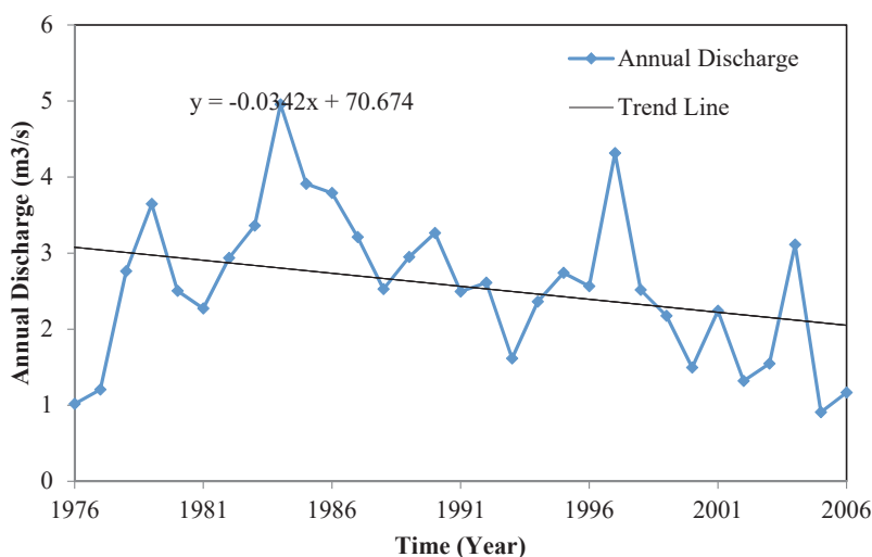
Fig. 2. The annual discharge changing trend of Soleimantangeh and Rigcheshmeh stations in the statistical period 1976–2006.
