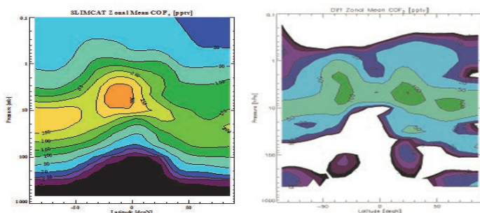
Fig. 13. SLIMCAT zonal mean of \text{COF}_2 , and the (MIPAS – SLIMCAT) difference in March 2010.
