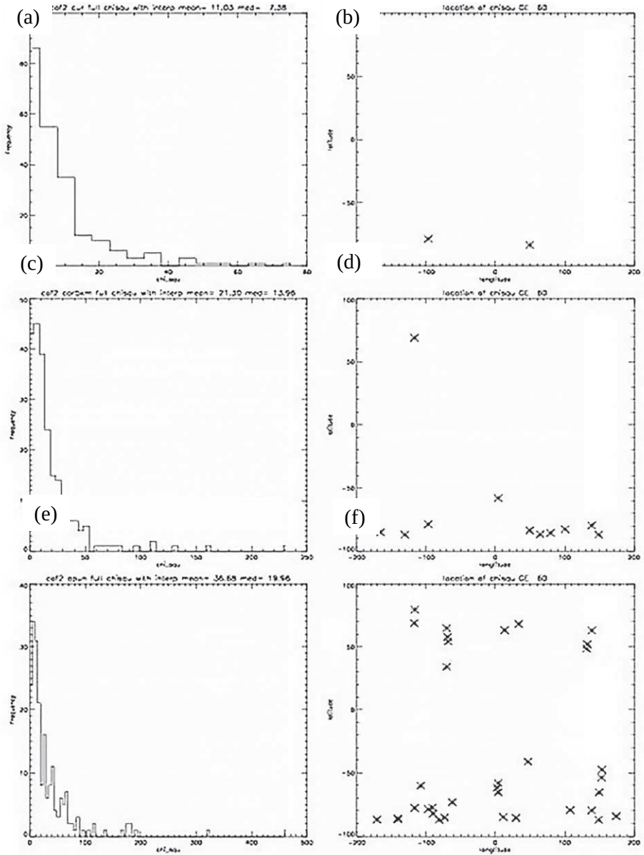
Fig. 25.(a), (c), and (e) are distributions of chi-square values with the band of 5 for the three different setting retrievals. The y axis is the frequency (i.e., number of counts) and the x axis is the chi-square value. (b), (d), and (f) are the locations of profiles that have chi-square value larger than the threshold of 60. The y axis is the latitude and the x axis is the longitude.
