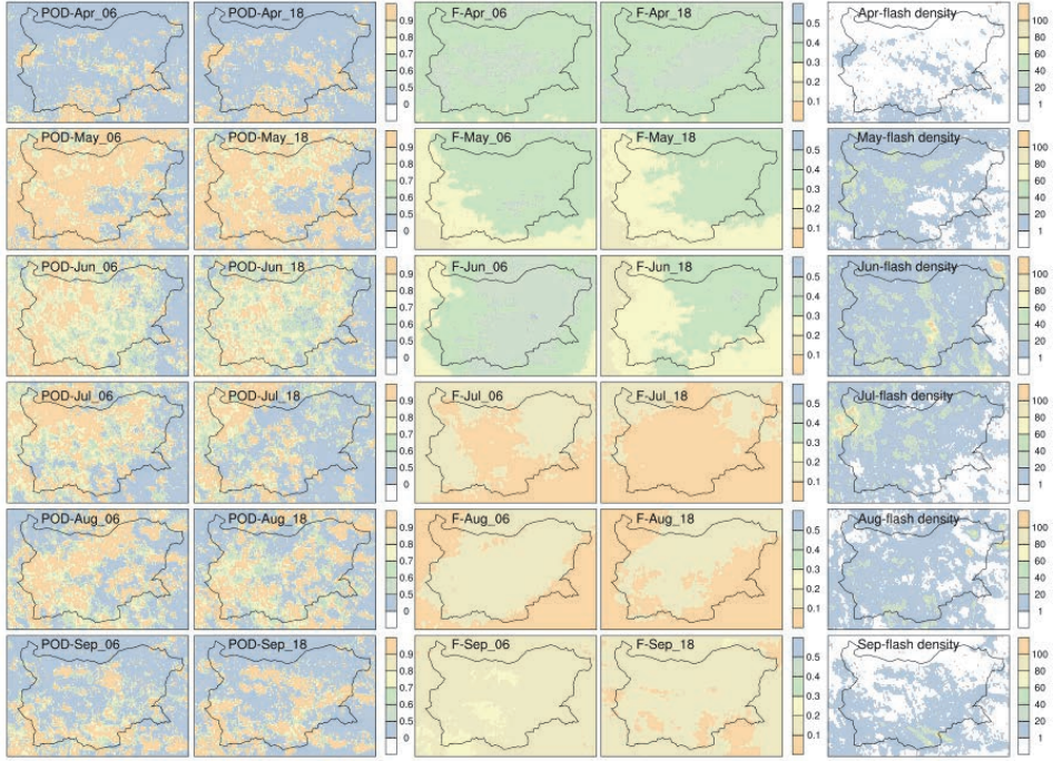
Fig. 11. 2021: Spatial distribution of probability of the detection (POD) and false alarm rate (F) for a grid of 5×5 km, for the model runs at 06 and 18 UTC (denoted respectively with “_06” and “_18”), and the flash density detected by ATDnet for the months April to September 2021 which is used to evaluate model forecast with a time frequency of 3 hours.
