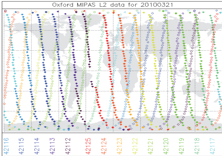
Fig.1. One day's sampling profile locations on March 21, 2010. Different colours represent different orbits with the number list below, while symbols are profile locations. Open symbols represent daytime measurements while solid symbols are nighttime measurements. (Source from http://www.atm.ox.ac.uk/group/mipas/L2OXF/20100321/ )
