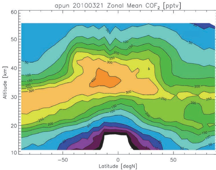
Fig. 19. Zonal mean of \text{COF}_2 with 1 day of data under “apun” setting, which changes the a priori uncertainty to 1000%.
