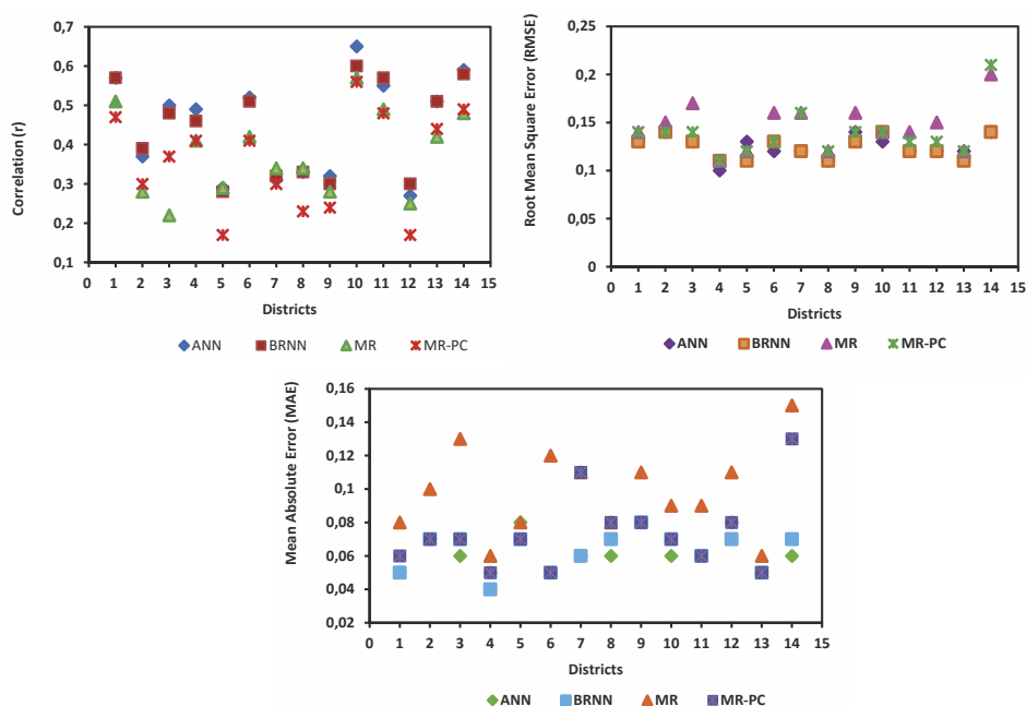
Fig. 7. Performance of ANN, BRNN, and multiple regression models for the test set (TRMM dataset).
