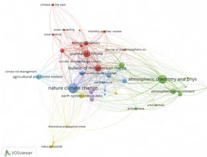
Fig. 2. Network visualization maps of citation journals in the field of meteorology and atmospheric sciences category based on WoS with 43 circles and 6 clusters.
