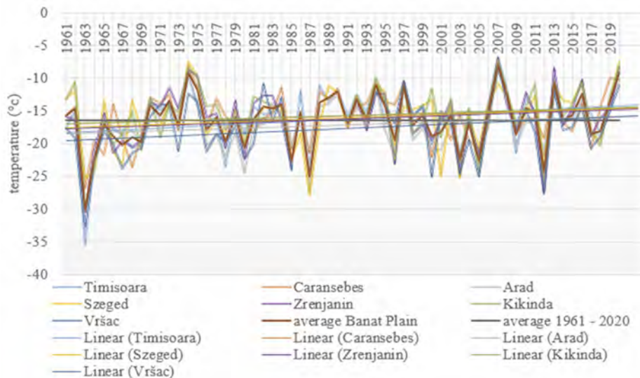
Fig. 13. Evolution of the annual minimum temperatures at the analyzed meteorological stations.
