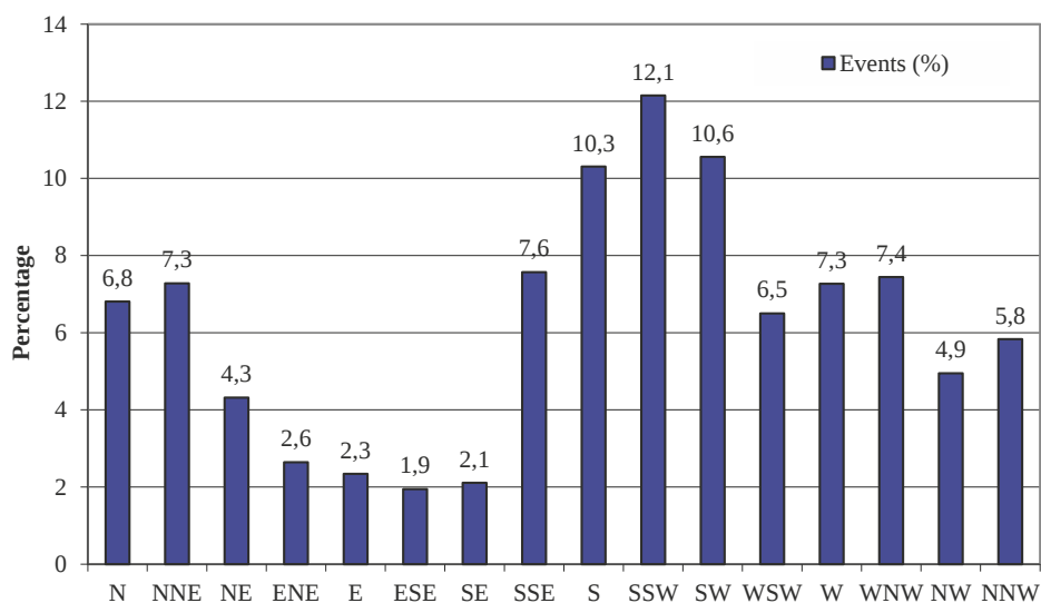
Fig. 4. Distribution of wind directions.
