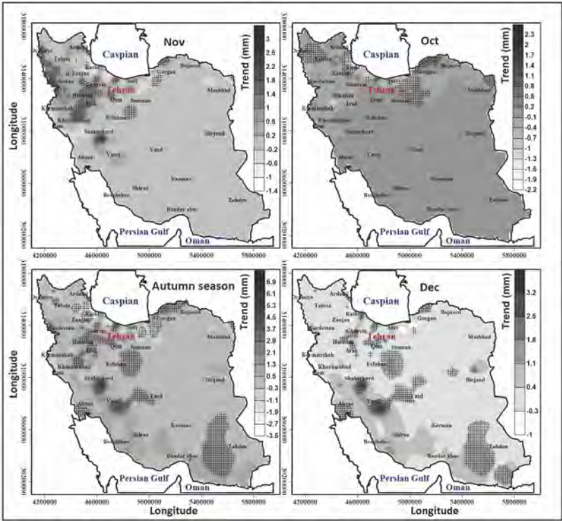
Fig. 3. Spatial distribution of the monthly trend of autumn precipitation in Iran.
