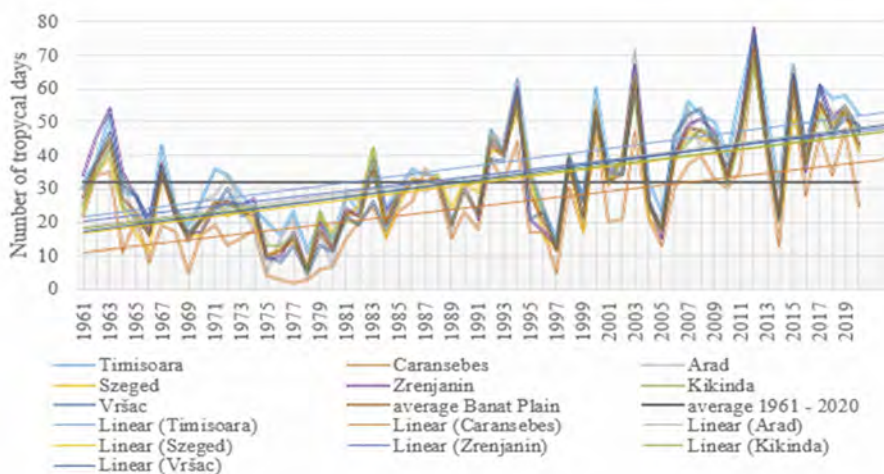
Fig. 2. Evolution of the annual number of tropical days at the analyzed meteorological stations.
