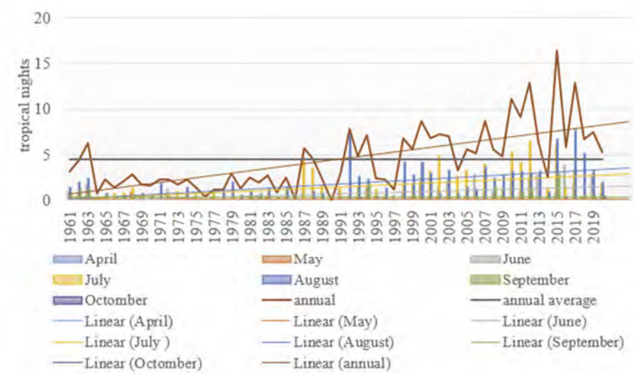
Fig. 8. Evolution of the monthly number of tropical nights in the Banat Plain.
