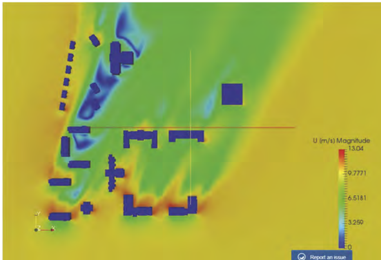
Fig. 10. Results of the CFD wind comfort analysis
