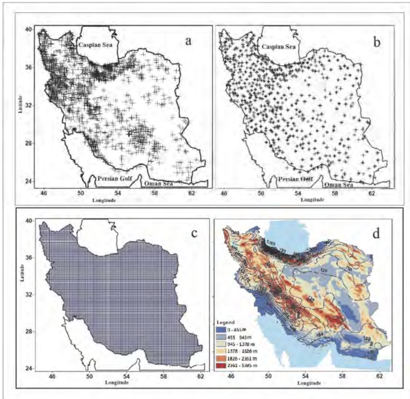
Fig. 1. Distribution of Al-Isfizari database (a), and distribution of supplementary stations (b), spatial resolution of NCEP/NCAR geopotential height data (c), and the calculated atmospheric thickness (d).
