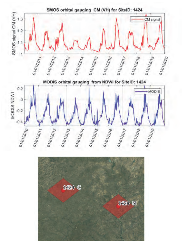
Fig. 5. Satellite river gauge derived from MODIS optical imagery and SMOS PMR data (upper two plots) for SGR 1424 (10.28°N, 1.05°W) over the White Volta River in Ghana. Lower map shows the location of PMR SGR for both M and C observation.
