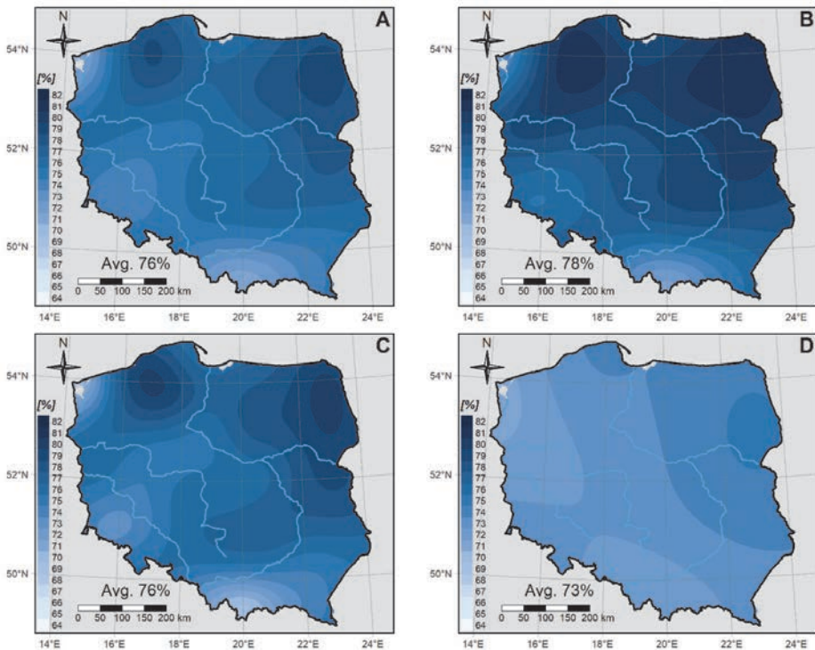
Fig. 4. Spatial distribution of the average cloudiness in winter (A), December (B), January (C), and February (D) in the years 1990/91–2019/20.
