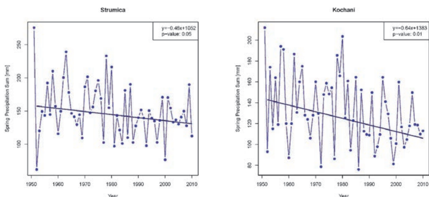
Fig. 3. SpPS series and statistically significant trends for Strumica and at Kochani with Sen's slope estimate and p-value.
