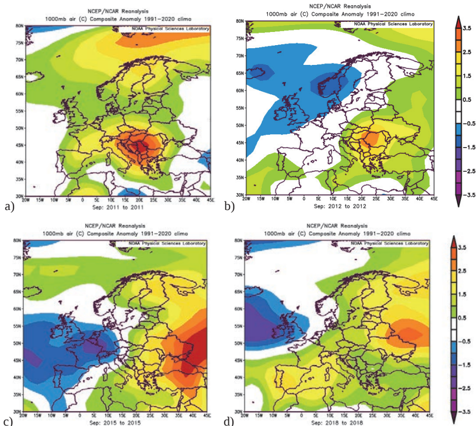
Fig. 11. Composite anomaly of 1000 hPa air temperature (°C) for: a) 2011, b) 2012, c) 2015, and d) 2018 compared to the period 1991–2020.
