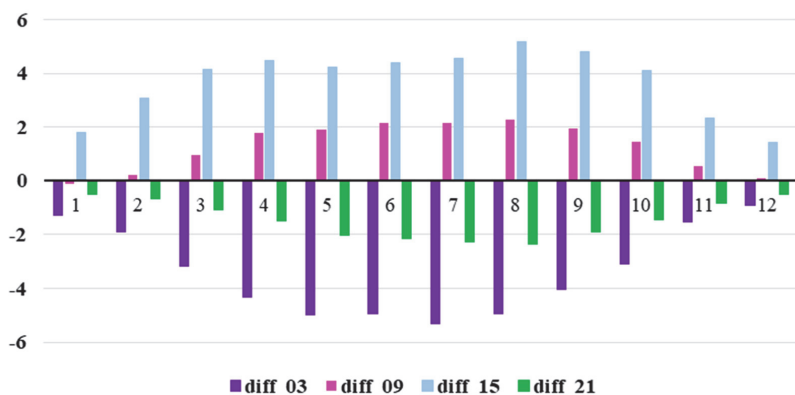
Fig. 2. Monthly difference of the six-hourly temperature values from the daily mean values (°C).
