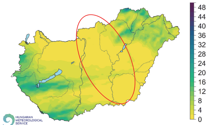
Fig. 9. 24-hour radar precipitation amount (July 13, 2023).
