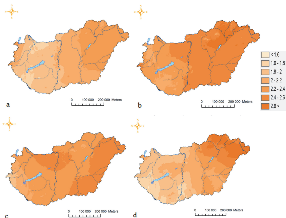
Fig. 10. The values of autumn change over the whole period (1971-2020), for hourly values (03 UTC (a), 09 UTC (b), 15 UTC (c), 21 UTC (d)), with linear trend estimation ( ^{\circ}\text{C} ). The change is significant at the 0.1 significance level in the entire area of Hungary.
