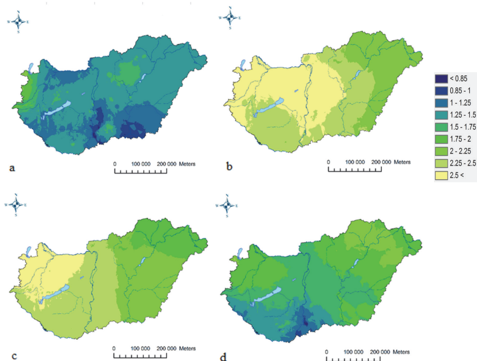
Fig. 8. The values of spring change over the whole period (1971-2020), for hourly values (03 UTC (a), 09 UTC (b), 15 UTC (c), 21 UTC (d)), with linear trend estimation (°C). The change is significant at the 0.1 significance level in the entire area of Hungary.
