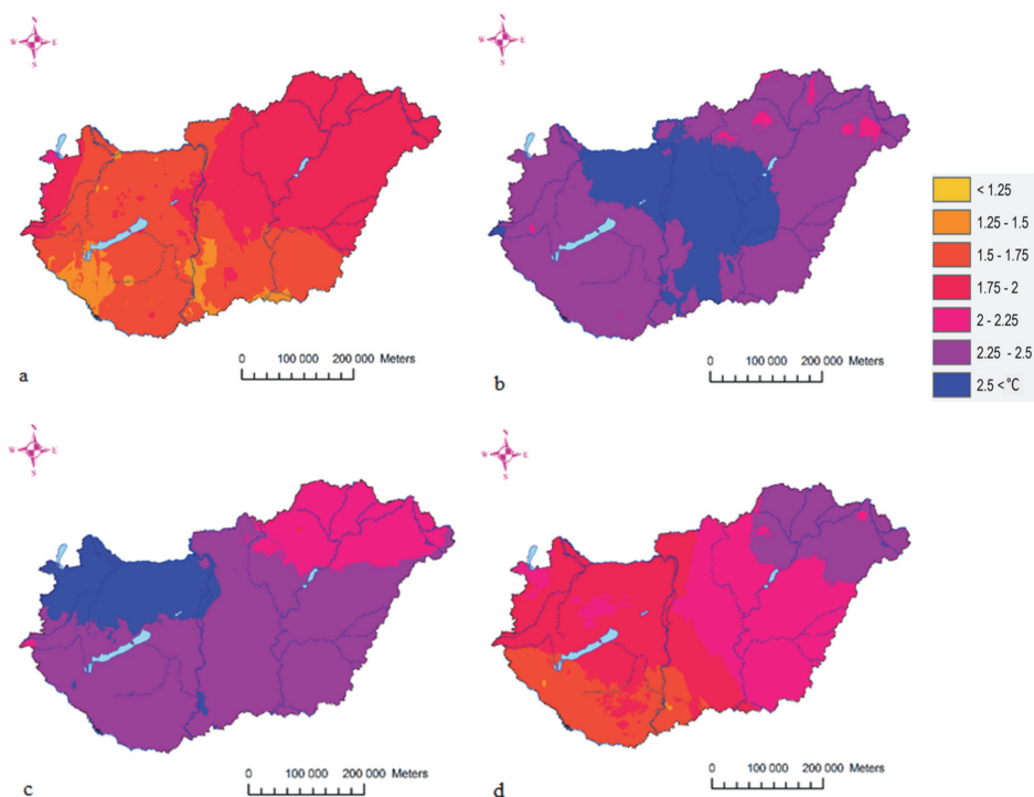
Fig. 7. The values of yearly change over the whole period (1971–2020), for hourly values (03 UTC (a), 09 UTC (b), 15 UTC (c), 21 UTC (d)), with linear trend estimation (°C). The change is significant at the 0.1 significance level in the entire area of Hungary.
