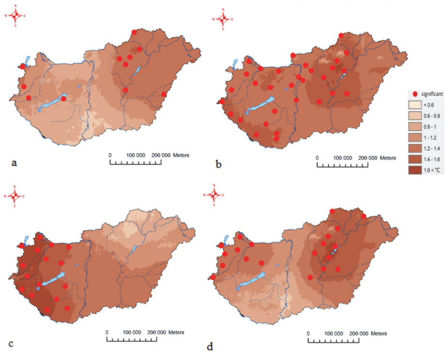
Fig. 11. The values of winter change over the whole period (1971-2020), for hourly values (03 UTC (a), 09 UTC (b), 15 UTC (c), 21 UTC (d)), with linear trend estimation (°C). Red points indicate the place of significant change at 0.1 significance level.
