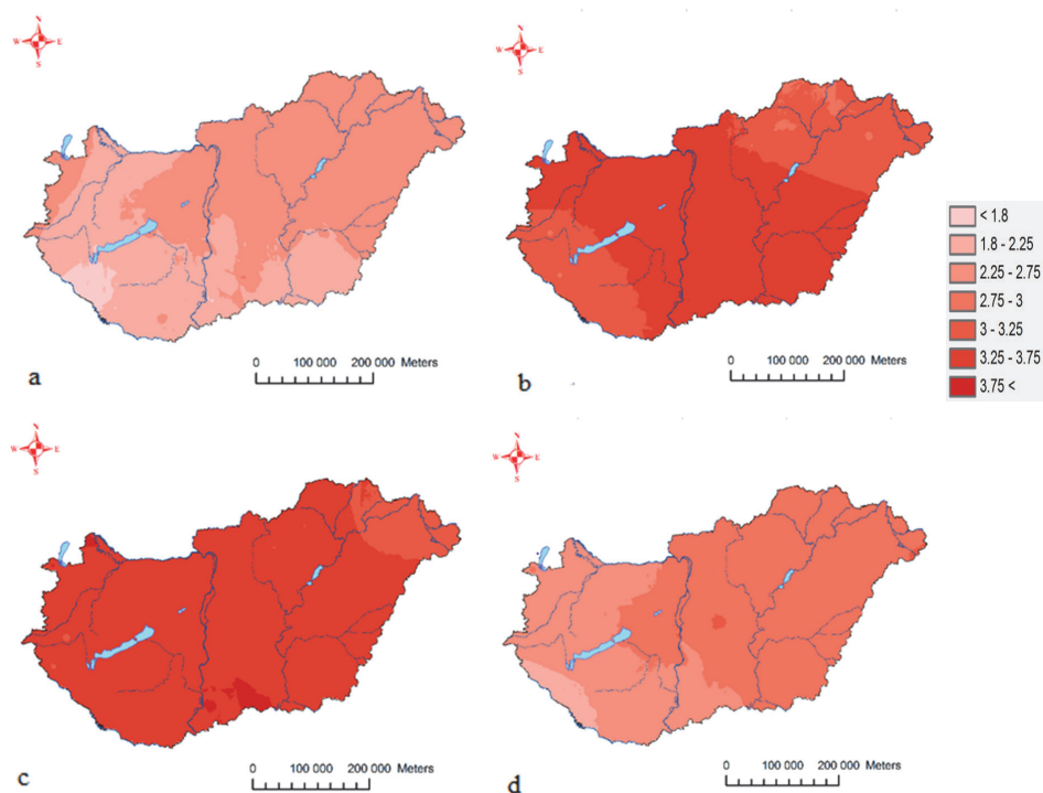
Fig. 9. The values of summer change over the whole period (1971-2020), for hourly values (03 UTC (a), 09 UTC (b), 15 UTC (c), 21 UTC (d)), with linear trend estimation (°C). The change is significant at the 0.1 significance level in the entire area of Hungary.
