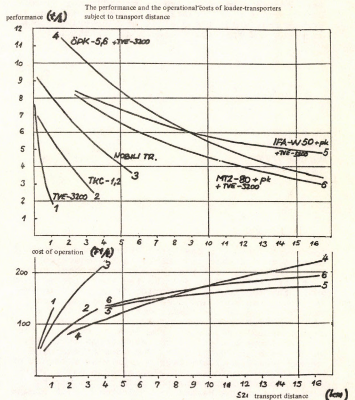
Figure 3 Changes in capacities and unit costs of fruit loading and transporting vehicles subject to transport distance
