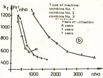
Figure 3 Specific characteristics of combines
