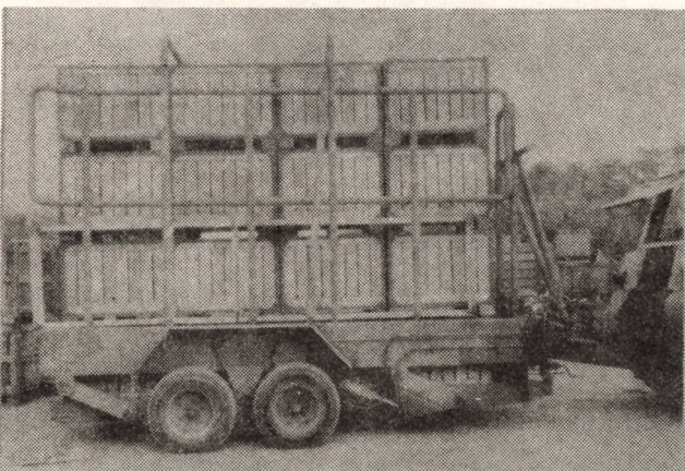
Figure 2 The Type ÖPK-5.6 self-loading fruit transporting trailer
