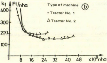
Figure 2 Specific characteristics of tractor
