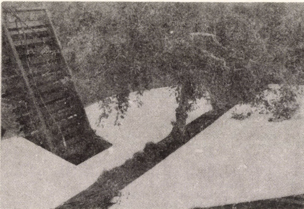
Figure 1 Continuous apple harvester, Type GSA
