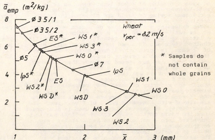
Fig. 2.: Effect of screen construction on grits fineness
