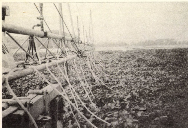
Fig. 2.: The flexible tubes for surface irrigation
