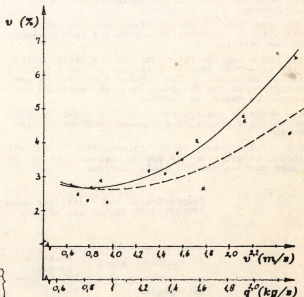
Fig. 2.: Loss parameters of the traditional and modified versions — traditional FKA adaptation - - - - - modified FKA adaptation
