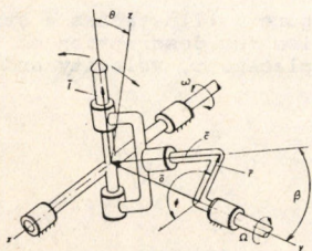
Fig. 4.: Crank axle oscillator
