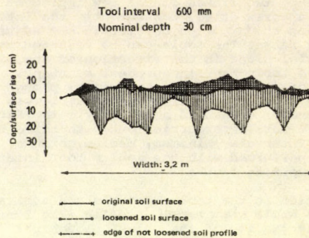
Fig. 4.: Transverse profile of the soil with maximum working depth
