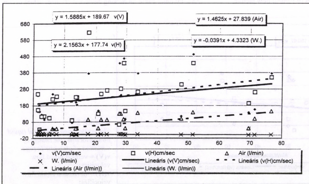
FIGURE 4 The air/liquid ratio likely to liquid velocity show an increasing trend v(V) = vertical liquid flow velocities; v(H) = horizontal liquid flow velocities; W = inlet of Water; Air = inlet of Air
