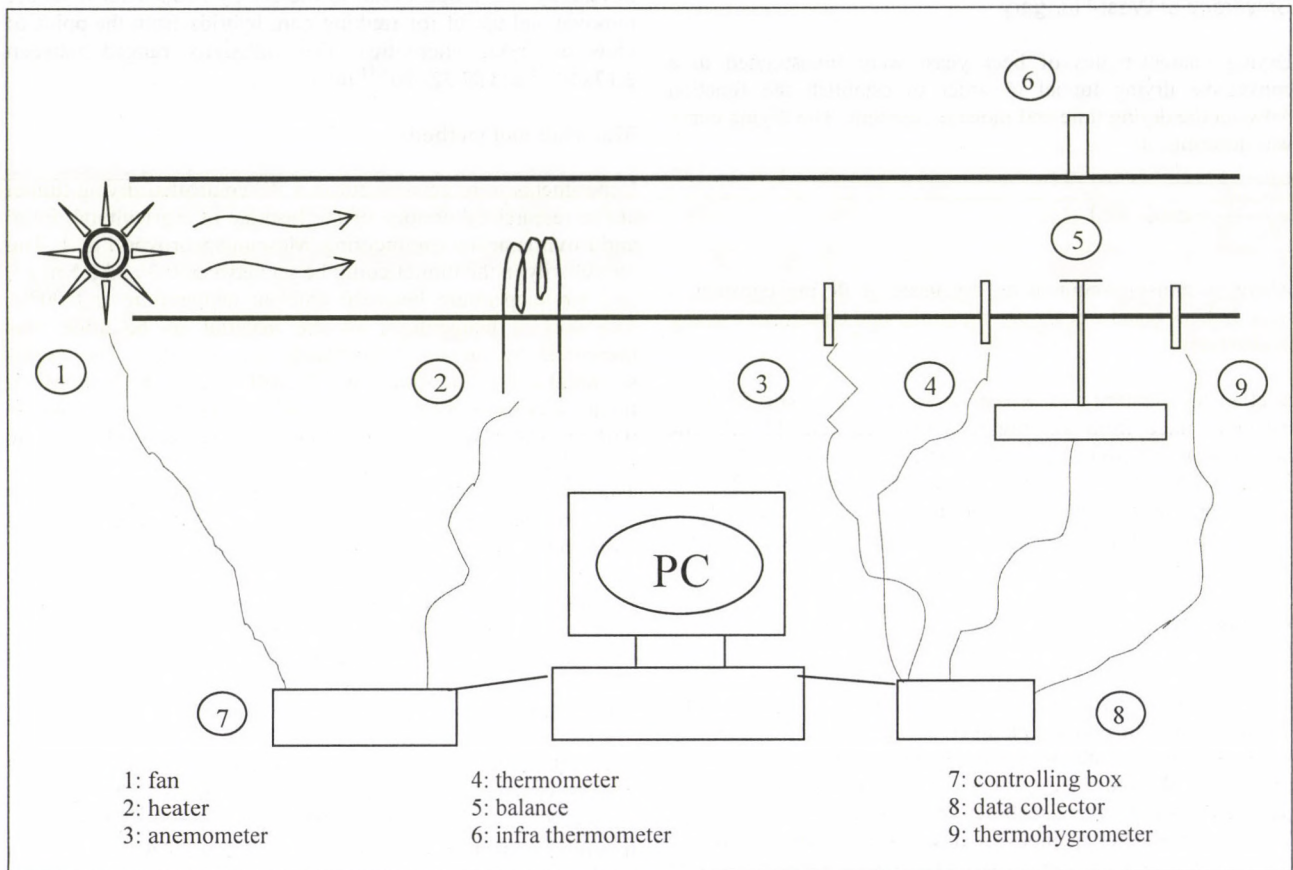
Figure 1 Experimental drying tunnel
