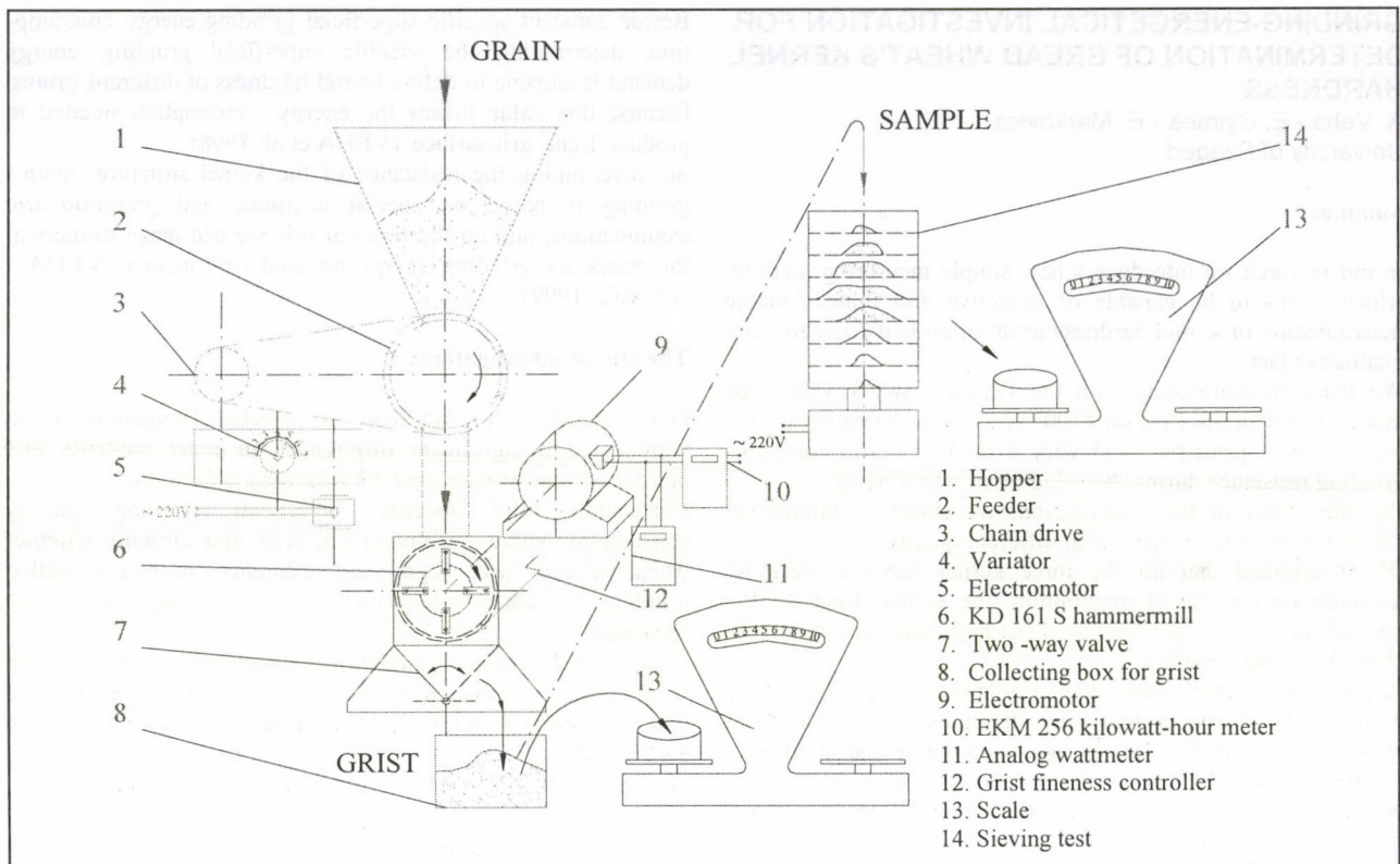
Figure 1 Measuring scheme of grinding resistance
