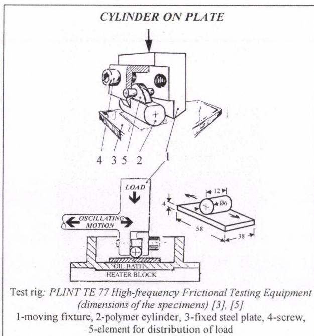
Figure 1 The equipment and the method [4]
