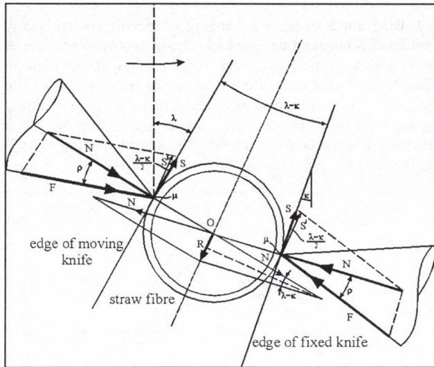
Figure 4 Determining borderline case of the scission
