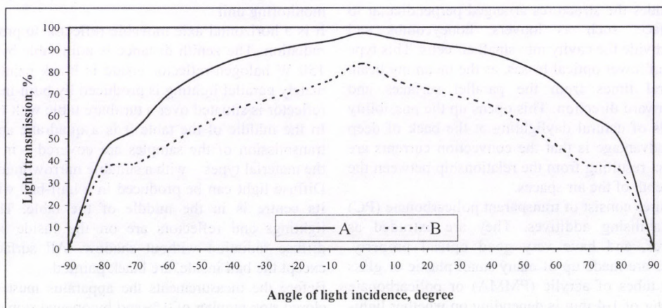
Figure 2 Light transmission factors for surface perpendicular structures (A: 40 mm thick capillary TI (polymetilmetakrilat, PMMA), B: 62 mm thick honeycomb TI material (Polycarbonat, PC)) [2]
