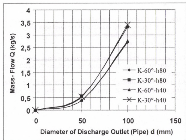
Figure 2 Measured mass-flow values in the function of discharge outlet diameters at corn outflow
