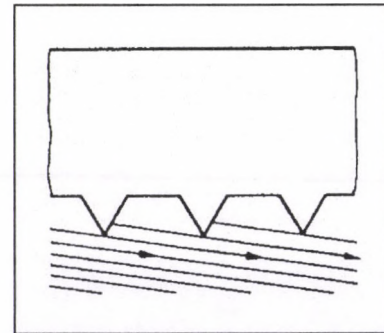
Figure 3 "Finesaw" affect originates from macroscopic surface roughness of the knife edge while scissoring
