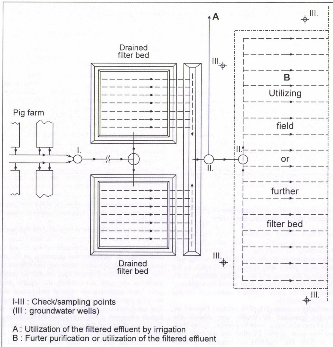
Figure 1 Slurry separation by soil filtration (soil filter beds + drained fields)
