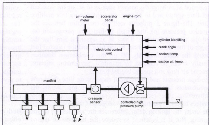
Figure 3 Electronic injection (Common Rail)
