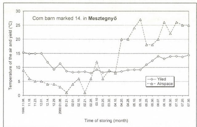
Figure 1 Changes of temperature in yield and air depending on duration of storing
