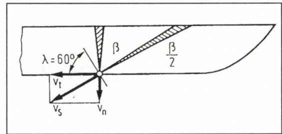
Figure 2 Decreasing of speed conditions and knife edge-angle while scissoring
