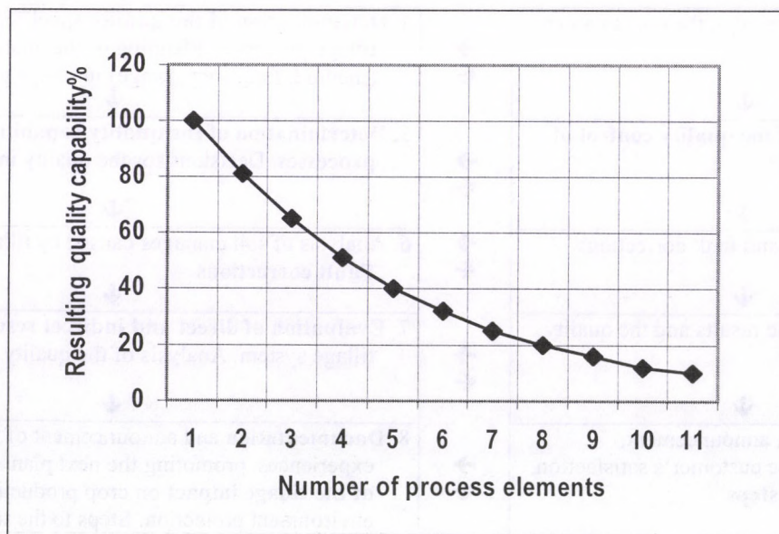
Figure 4 Resulting quality capability in the process series if the capability of the process elements has 90 % rate
