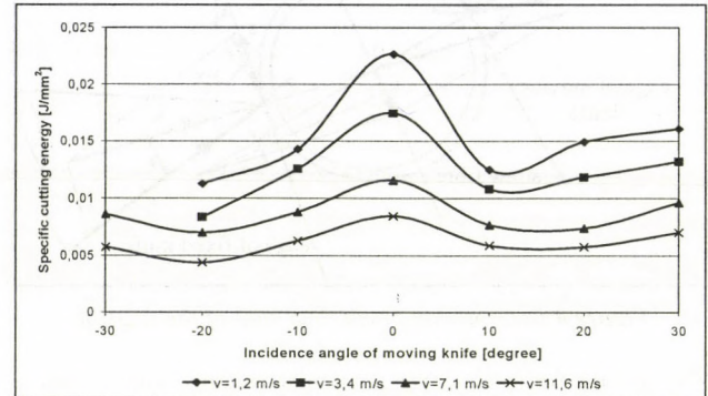
Diagram 3 Specific cutting energy plotted against the incidence angle of moving knife (Kisvárdá 63 rye; w=34\% ; a=10 mm, fixed knife 0°)
