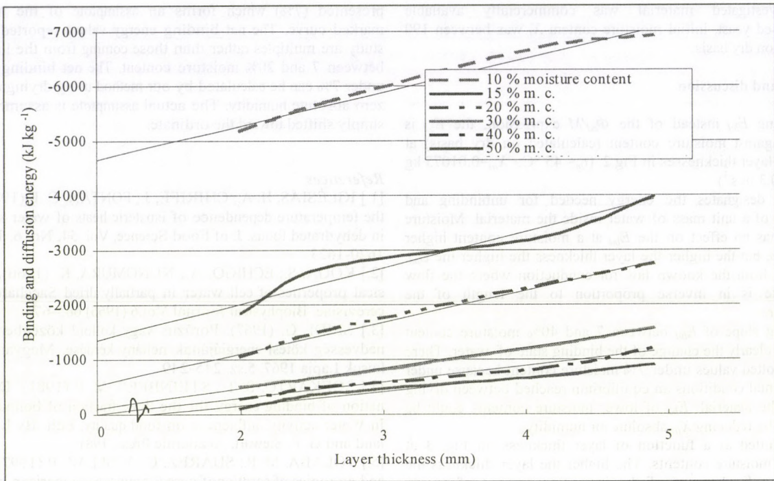
Figure 3 E_{bd} vs. layer thickness at different moisture content
