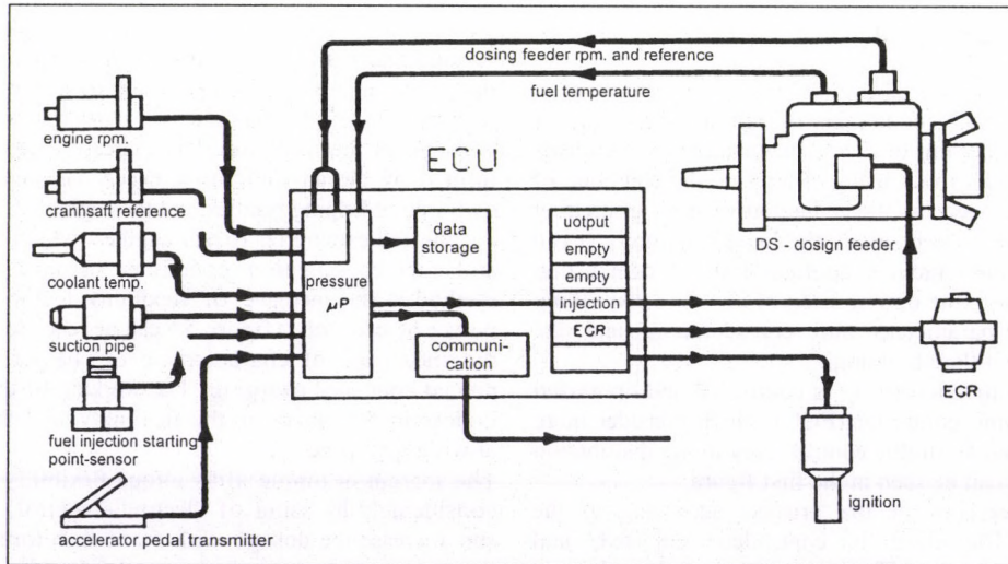
Figure 1 Electronic controlled injection system (ECU)
