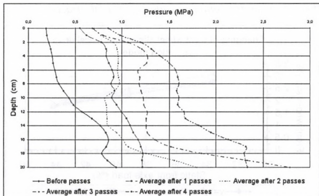
Figure 5 Soil compaction after passes
