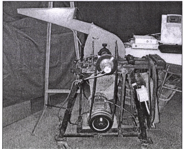
Fig. 1 Zenit Junior hammer mill
