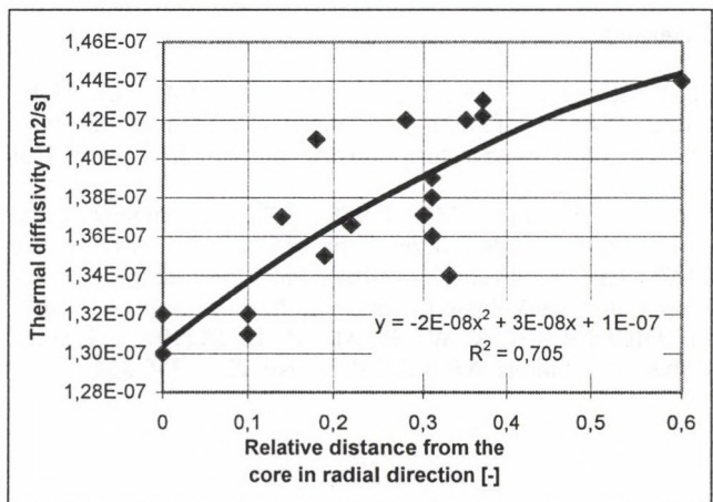
Fig. 3 Effect of temperature sensor placement error on the thermal diffusivity for Parisers (d=80 mm)
