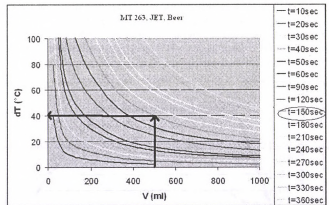
Fig. 6 Temperature increase as a function of volume
