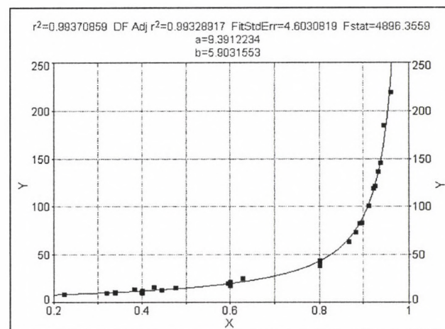
Fig. 6 Determination of desorption equation of carrot (24 °C)
