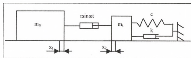
Fig. 2 Mechanical model of the vibration-system
