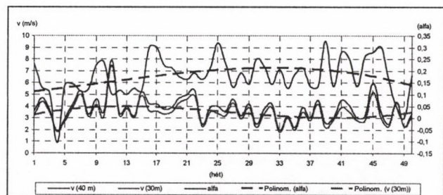
Fig. 8 Course of the alpha coefficient and the average wind speeds during 1 year on a good orographic place
