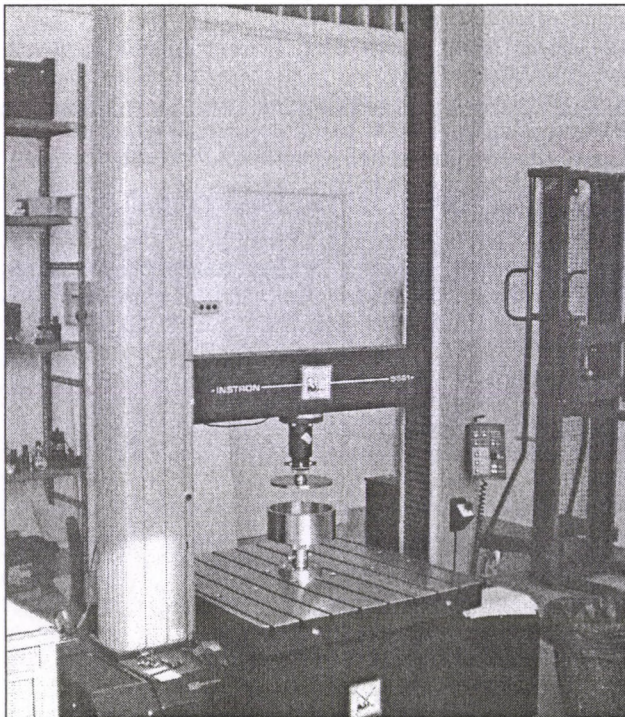
Fig. 1 Instron-5581 type tester
