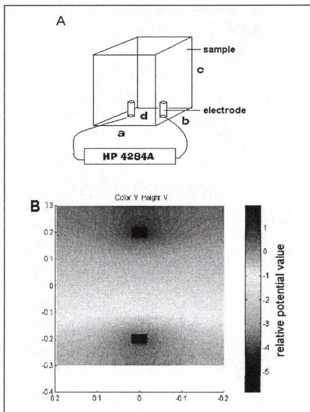
Fig. 1 A Electrode arrangement in apple and potato slices with a , b and c edges. d is the distances between the two electrodes.
