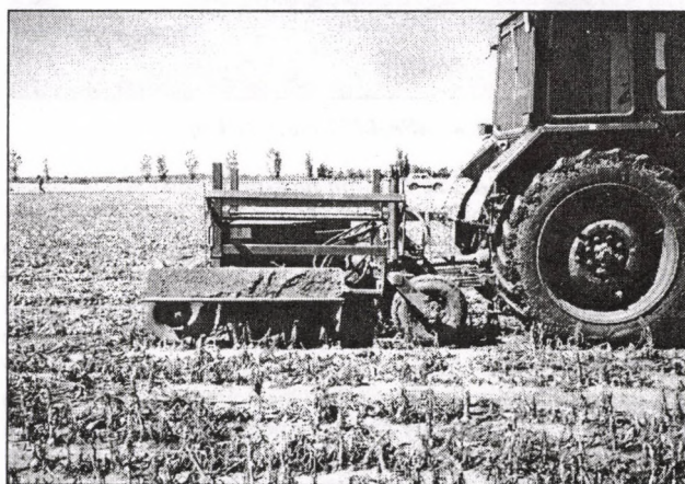
Fig. 2 ASA-LIFT haulm cutter
