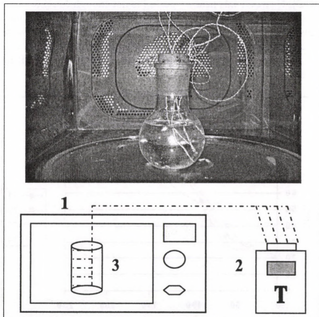
Fig. 2 Periodical heating
