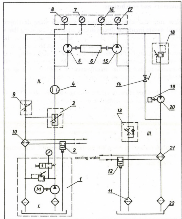
Fig. 1 The hydrostatic test bench
