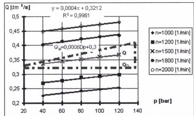
Fig. 2 Input flow curves of the examined hydro-motor
