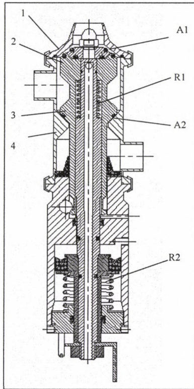
Fig. 1 The cutaway view of valve
