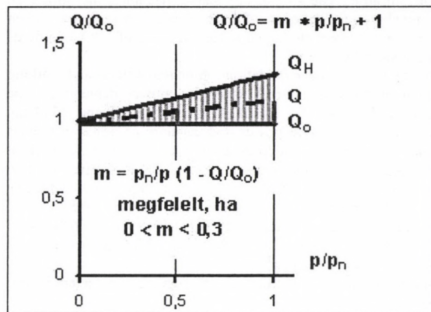
Fig. 3 Determination of the technical condition of hydro-motors
