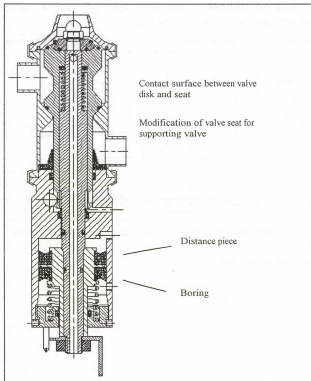
Fig. 4 The cutaway view of the modified valve
