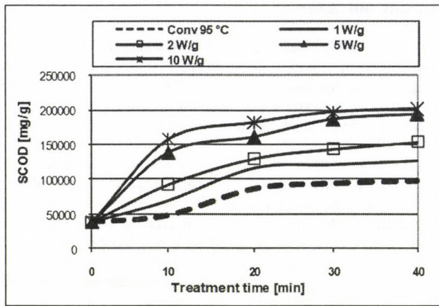
Figure 1 The changes of solubility of organic matter content after microwave and convective treatments
