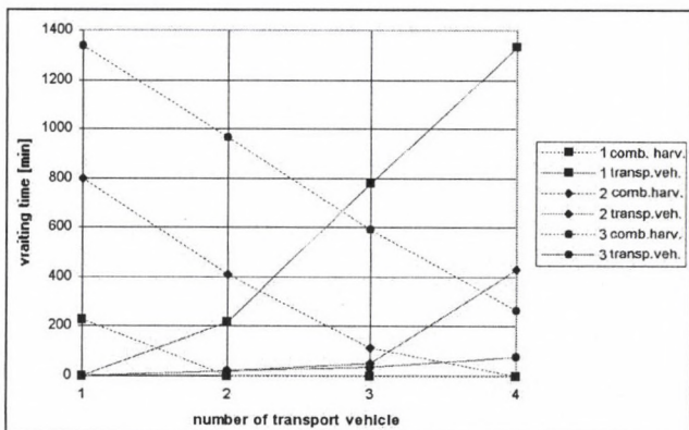
Figure 5 Connection between the waiting time, number of transport vehicles and combine harvesters
