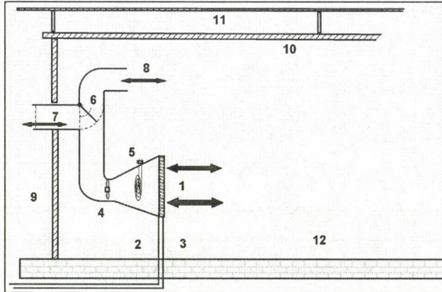
Figure 6 The suggested construction design 1 – air-water heat exchanger, 2 – inlet from the soil collector, 3 – outlet towards the soil collector, 4 – reversible fan of variable rotary speed, 5 – auxiliary heater, 6 – changeover air flap; 7 – inlet/outlet opening of external air, 8 – inlet/outlet opening of internal air, 9 – insulated side wall of the container, 10 – insulated ceiling of the container, 11 – shade from the sun
