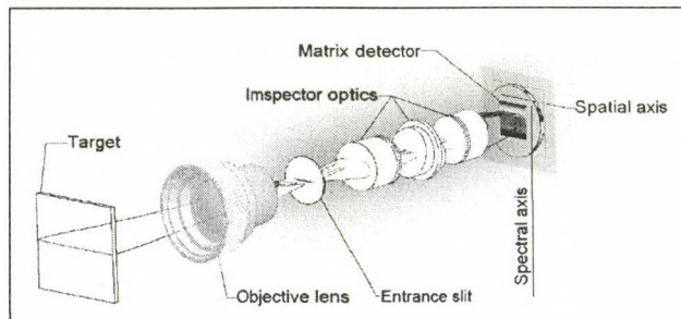
Figure 1 The spectrograph
