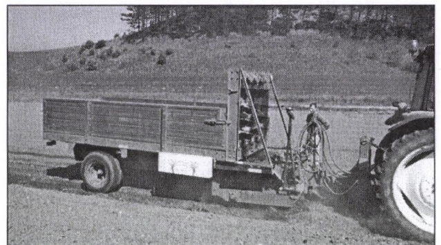
Figure 1 Rhizome planter NORDIC (Hvidsted Energy Forest)
