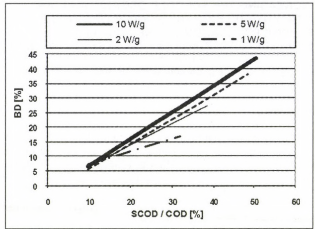
Figure 3 Connection between solubility and biodegradability
