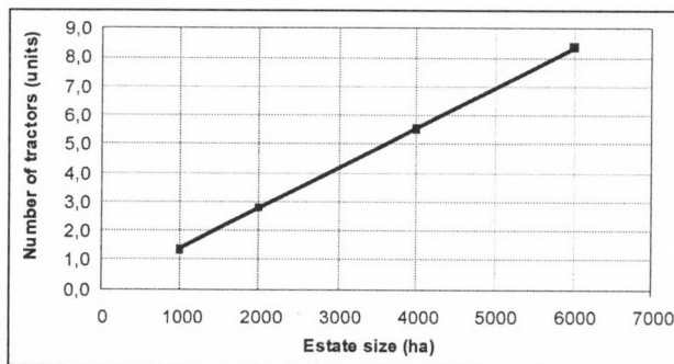
Figure 2 Relation between estate size and the required number of tractors of the 40 kN category, k_s=0.8 \text{ daN/cm}^2 , L=800 \text{ ha}
