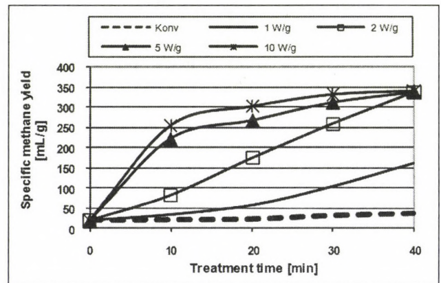
Figure 4 Specific methane yield after microwave pretreatments
