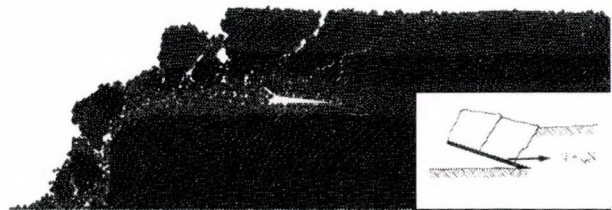
Figure 7. Side view of the loosening and clod generation by DEM and the theoretic aspect (SITKEI 1967)
