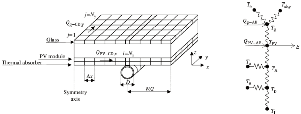
Figure 3. Sketch of the discretization used for the thermal analysis (left) and network of thermal resistances on the x-z plane between the layers of the PVT module (right) [13]
