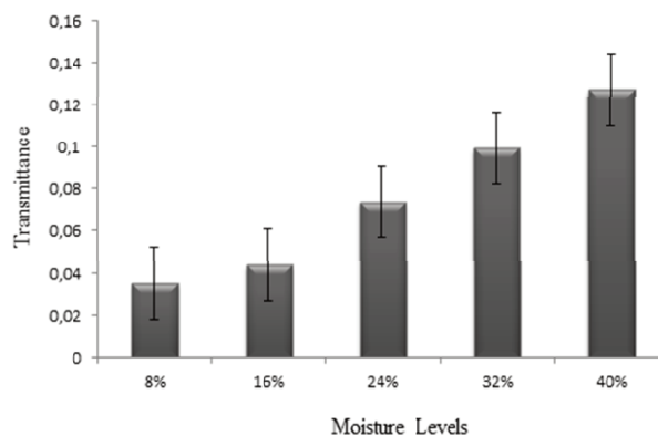
Figure 3. Transmittance trend of yellow tigernut influenced by moisture
