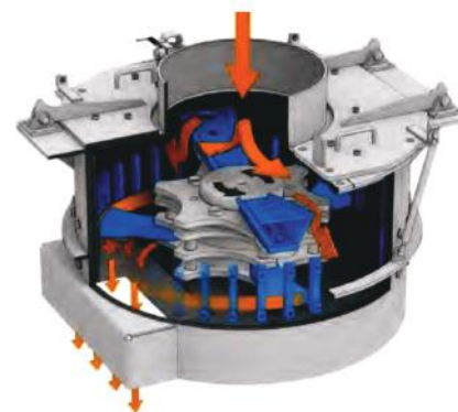
Figure 1. The BHS Biogrinder RBG 08 parts
