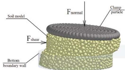
Figure 2. Numerical direct shear tests.
