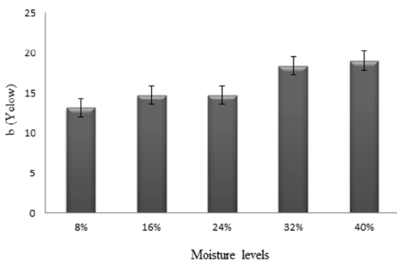
Figure 7: b(Yellow) trend
