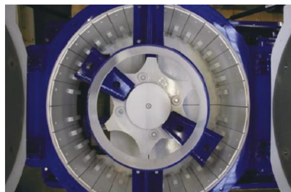
Figure 3. The turning and fix parts view from top
