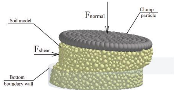
Figure 2. Numerical direct shear tests.
