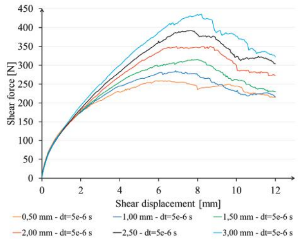
Figure 7. Effect of the Bond radius.
