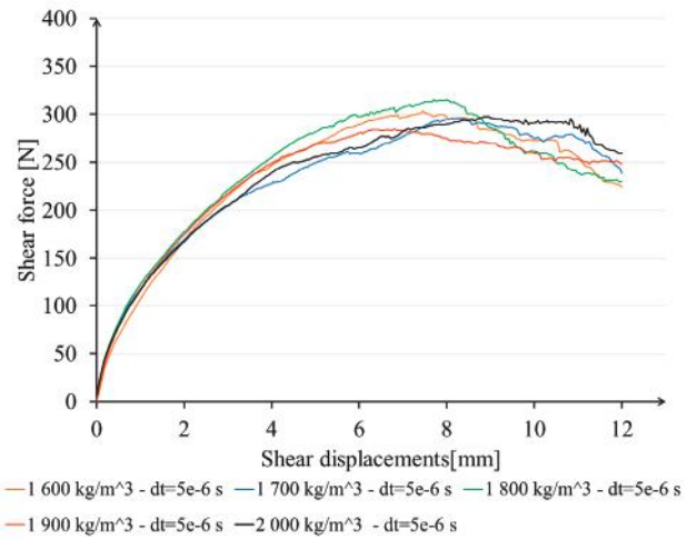
Figure 6. Effect of the particle's density.
