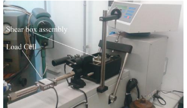
Figure 1. The ELE 26-2112/01 type direct shear apparatus.
