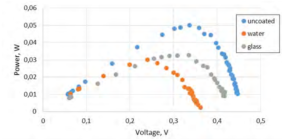
Fig. 5. P-V characteristics
