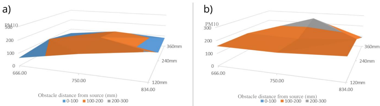
Figure 3. graphs of Average PM10 concentration registered by Sensor A in the function of Obstacle heights and distance from the source in case of a) wind speed 2.9 m/s and b) wind speed 1 m/s
