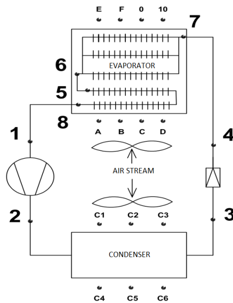
Figure 5. The measurement system and measurement locations
