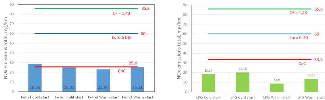
Figure 8. Vehicle NO x emission when fuelled with petrol (blue) and LPG (green)
