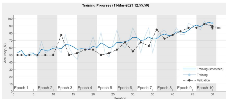
Figure 6. Evolution of accuracy over training epochs for the entire face detection.
