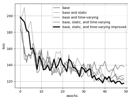
Figure 19 Loss function evolution on the validation data across the epochs
