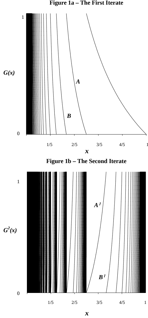
Figure 1: Symmetry Partners between the First and Second Iterates of the Gauss Map
