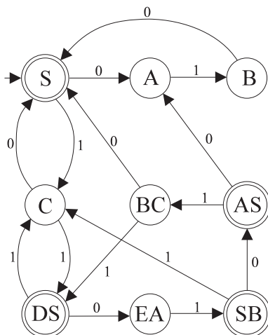
FIGURE 2. Automaton \mathcal{A}_D(010, 1101, 10, 11)
