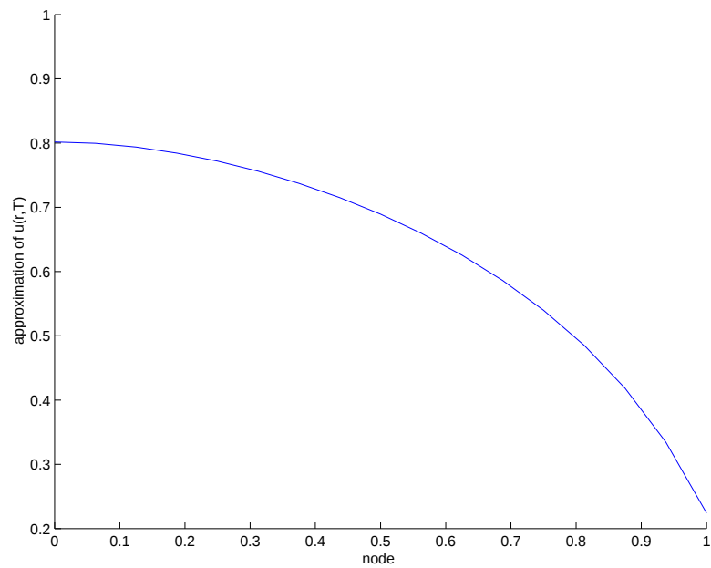
FIGURE 5. Profile of the approximation of u(r, T) , where T is the quenching time \varepsilon = 0
