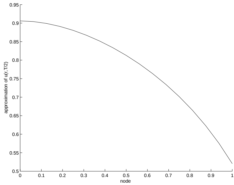
FIGURE 4. Profile of the approximation of u(r, T/2) , \varepsilon = 0
